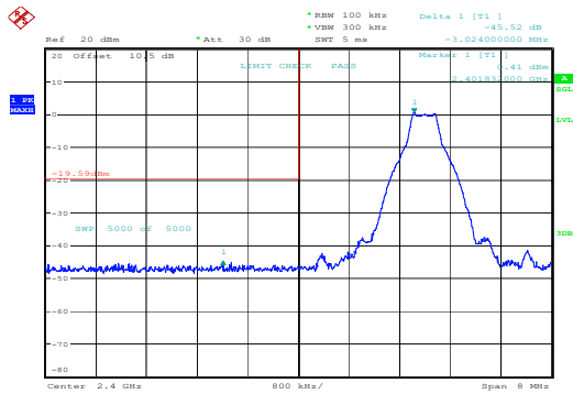
GFSK_Low
