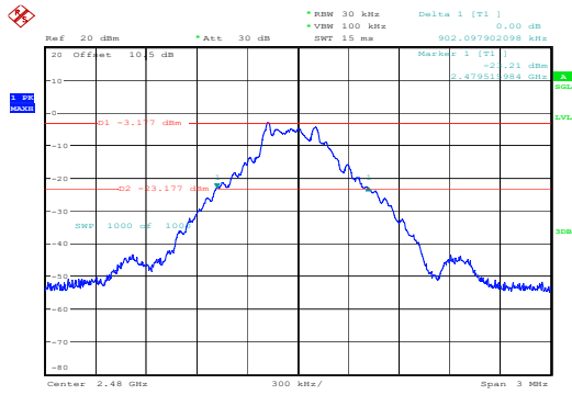
GFSK_High 0.902MHz
