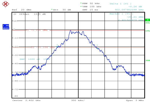
GFSK_Low 0.902MHz
