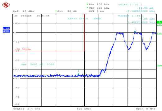
GFSK_Hopping_Lower
