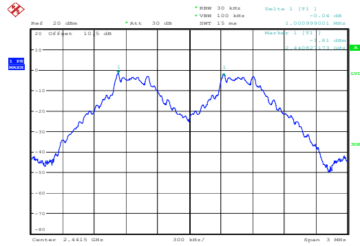
GFSK_Middle 1.001MHz
