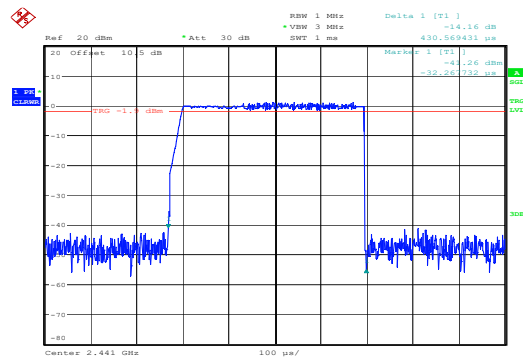
\pi/4 -DQPSK_Hopping_2DH1 0.431ms
