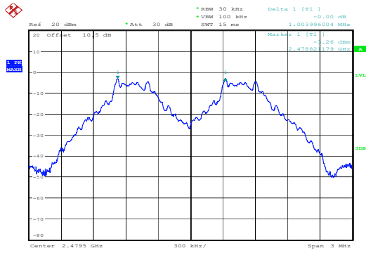
GFSK_High 1.004MHz
