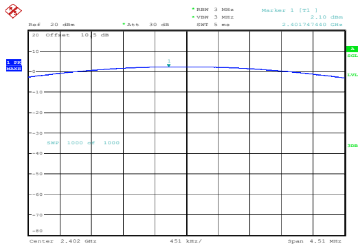
GFSK_Low2.10dBm
