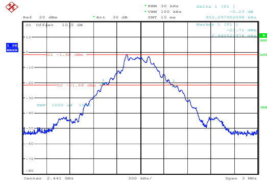
GFSK_Middle 0.902MHz
