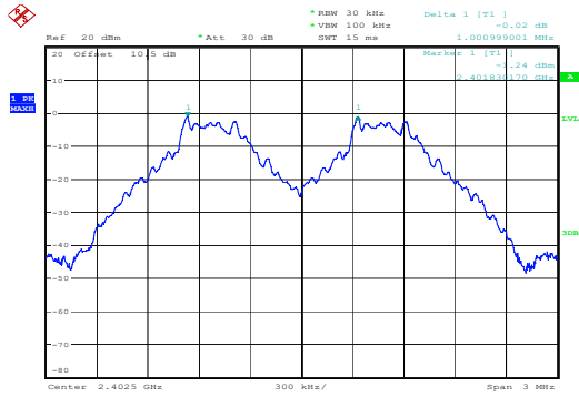
GFSK_Low 1.001MHz
