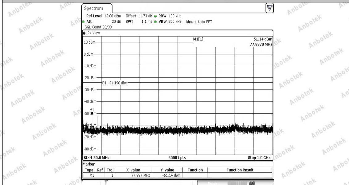
3DH5-Ant1-2480-30~1000-PASS
