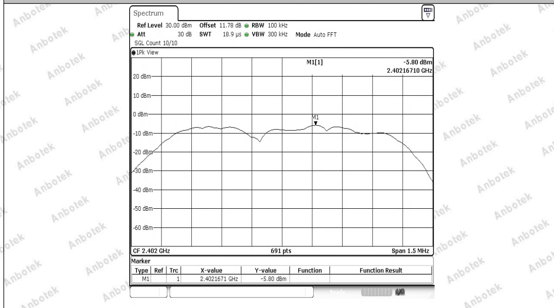
2DH5-Ant1-2402-0~Reference-PASS
