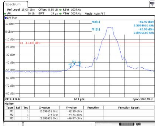
GFSK LOW CHANNEL, BAND EDGE
