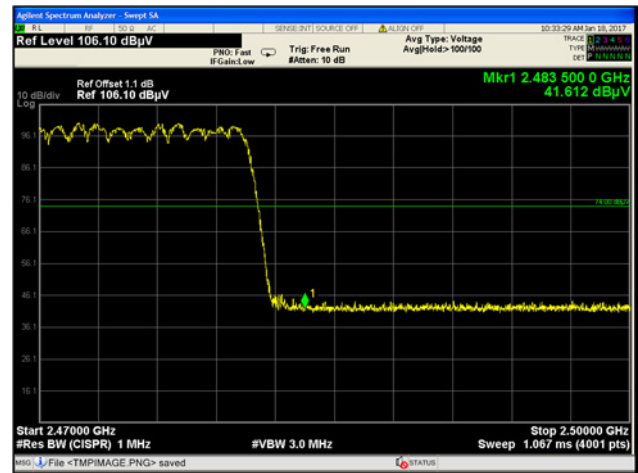
8-DPSK HIGH FREQUENCY BAND, PEAK
