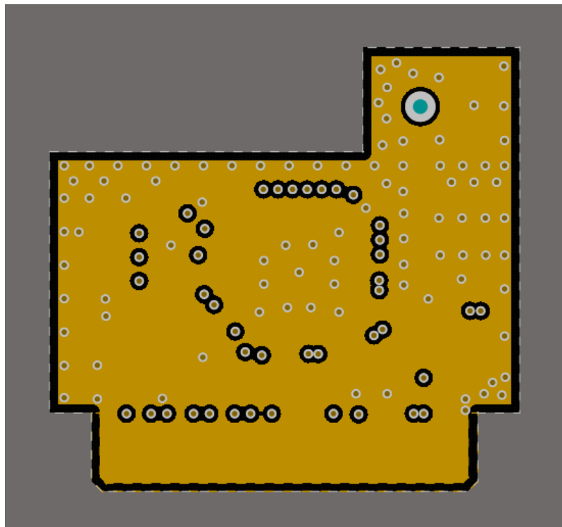
Figure 2 ESP-01E PCB GND Layer
