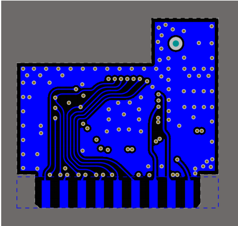
Figure 4 ESP-01E PCB Bottom Layer
