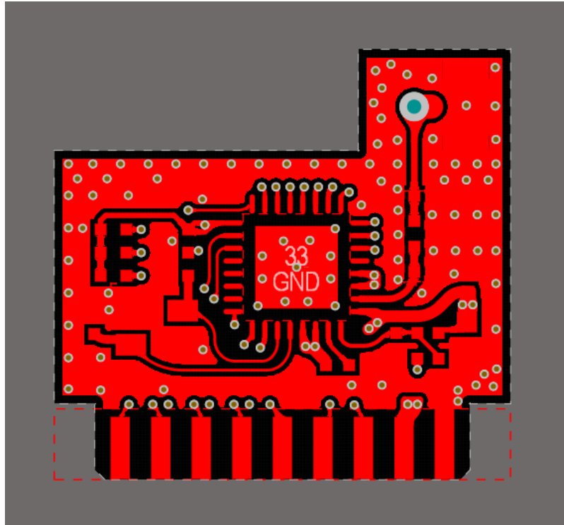
Figure 1 ESP-01E PCB Top Layer
