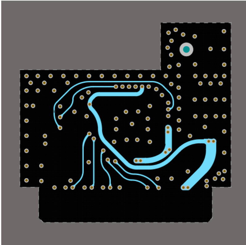
Figure 3 ESP-01E PCB POWER Layer
