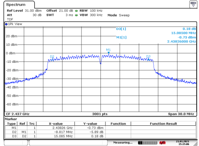
Figure 8.8-2: PSD on mid channel
