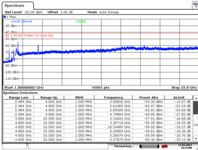
Figure 8.7-13: Conducted spurious emissions above 1 GHz within restricted bands, Tx on low channel
