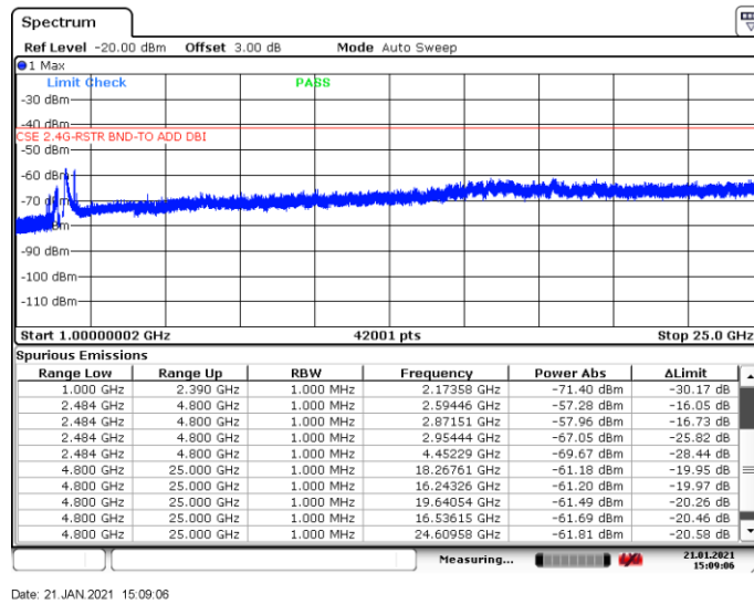
Figure 8.7-15: Conducted spurious emissions above 1 GHz within restricted bands, Tx on high channel
