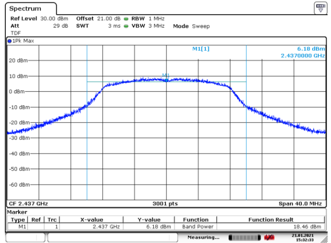
Figure 8.6-2: Output power on mid channel
