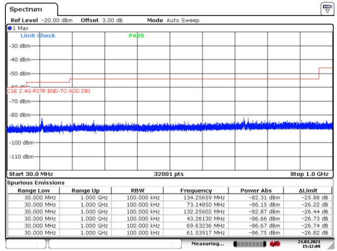
Figure 8.7-11: Conducted spurious emissions 30 MHz to 1 GHz within restricted bands, Tx on mid channel
