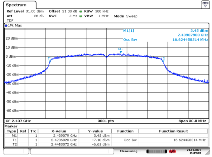
Figure 8.5-5: 99% bandwidth on Mid Channel
