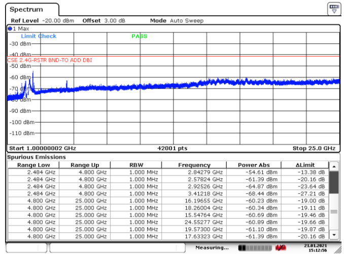
Figure 8.7-14: Conducted spurious emissions above 1 GHz within restricted bands, Tx on mid channel
