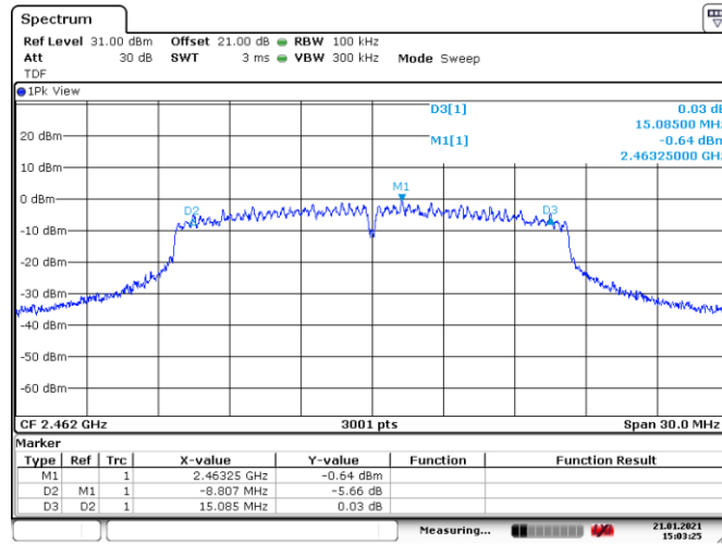
Figure 8.8-3: PSD on high channel
