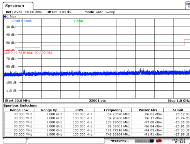
Figure 8.7-12: Conducted spurious emissions 30 MHz to 1 GHz within restricted bands, Tx on high channel
