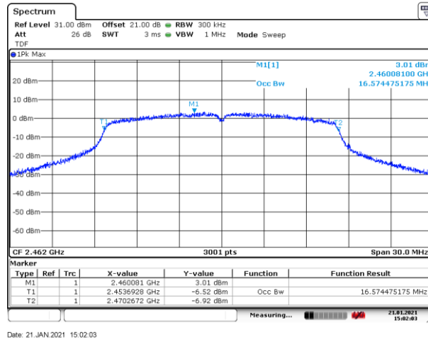
Figure 8.5-6: 99% bandwidth on High Channel
