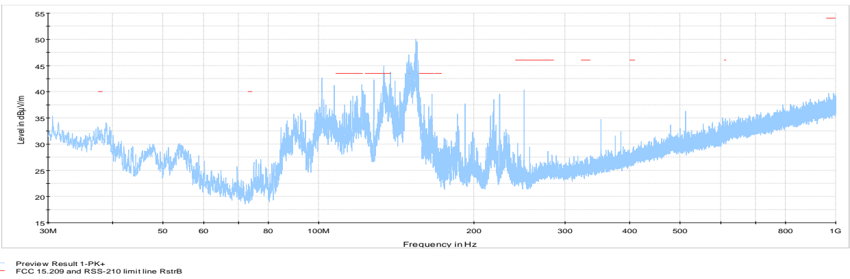
Figure 8.7-17: Cabinet radiated Spurious emissions within 30 to 1000 MHz, Tx @ mid channel
