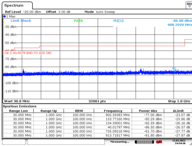
Figure 8.7-10: Conducted spurious emissions 30 MHz to 1 GHz within restricted bands, Tx on low channel
