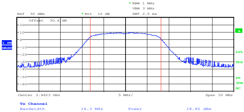
Figure 8.3-3: output power plot on High channel
