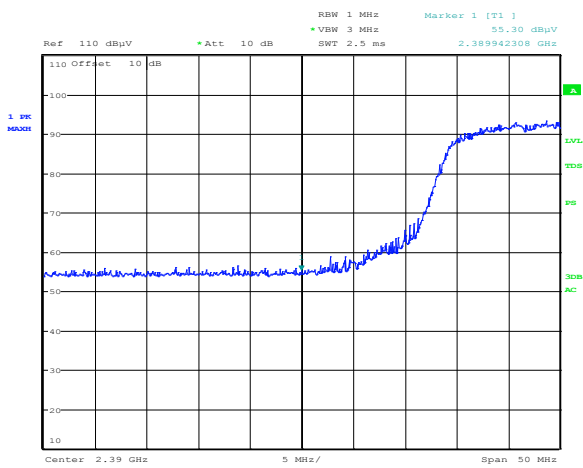
Figure 8.4-1: Conducted Band edge emission, low channel
