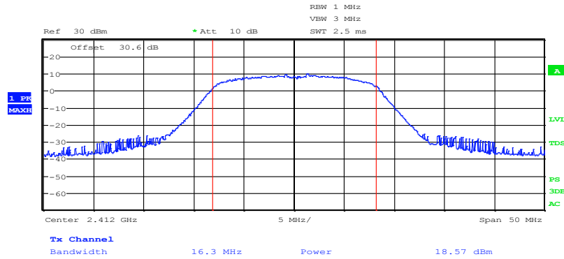
Figure 8.3-1: output power plot on Low channel
