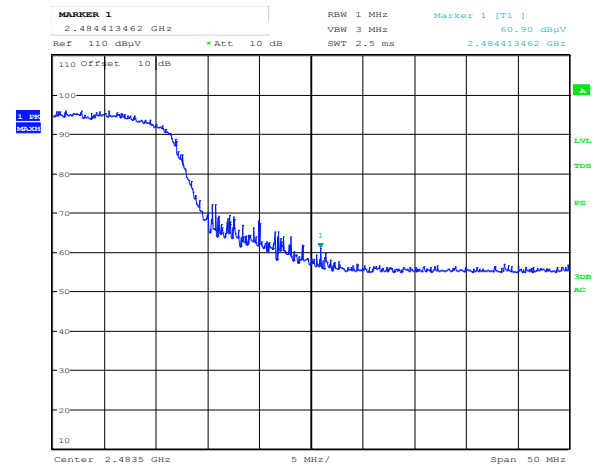
Figure 8.4-2: Conducted Band edge emissions for high channel
