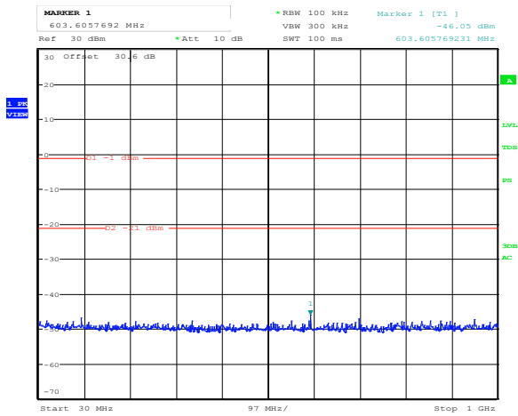
Figure 8.4-5: Conducted spurious emissions, Low channel_30MHz – 1GHz
