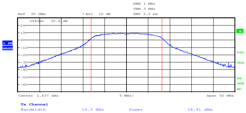
Figure 8.3-2: output power plot on Mid channel
