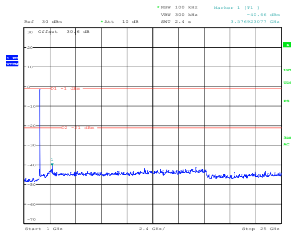
Figure 8.4-6: Conducted spurious emissions, Low channel_1 GHz – 25GHz
