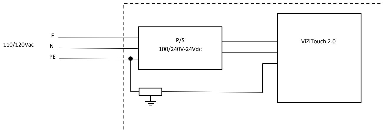
Figure 3.6-1: Setup diagram
