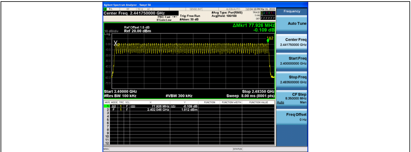
GFSK Modulation
