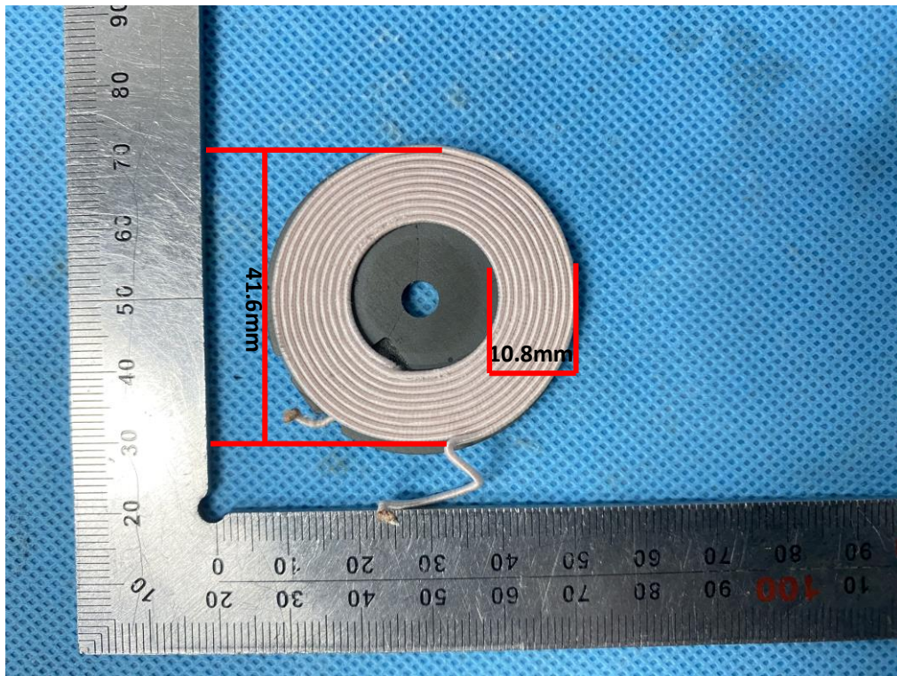
WPT ANTENNA
