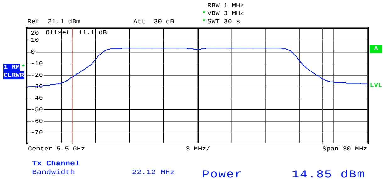
Plot 2.1 802.11a, 5500MHz
