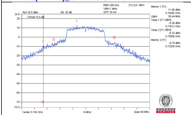
802.11ac(VHT20)_Chain2 / CH149
