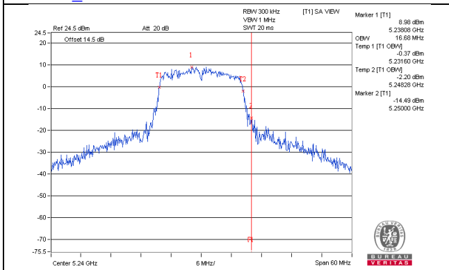
802.11ac(VHT20)_Chain0 / CH48
