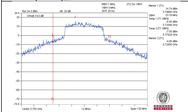
802.11ac(VHT40)_Chain2 / CH151
