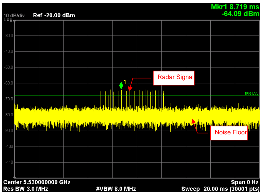
Radar Signal 2
