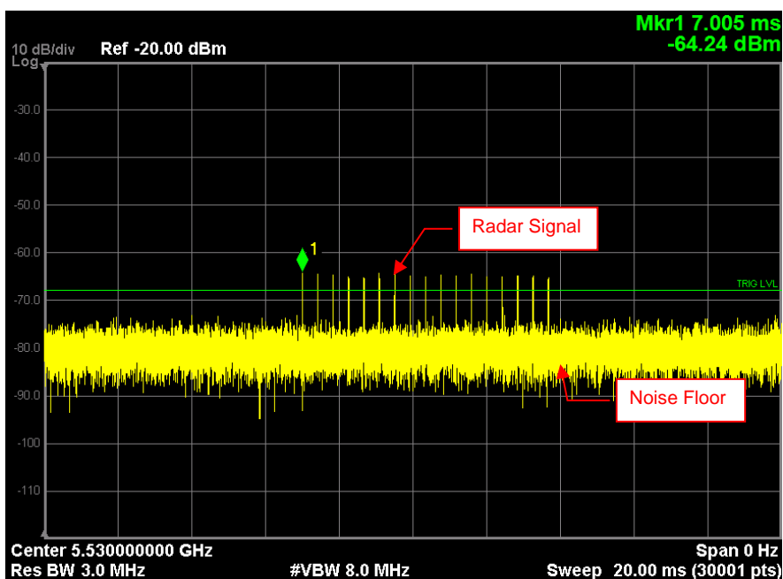
Radar Signal 3
