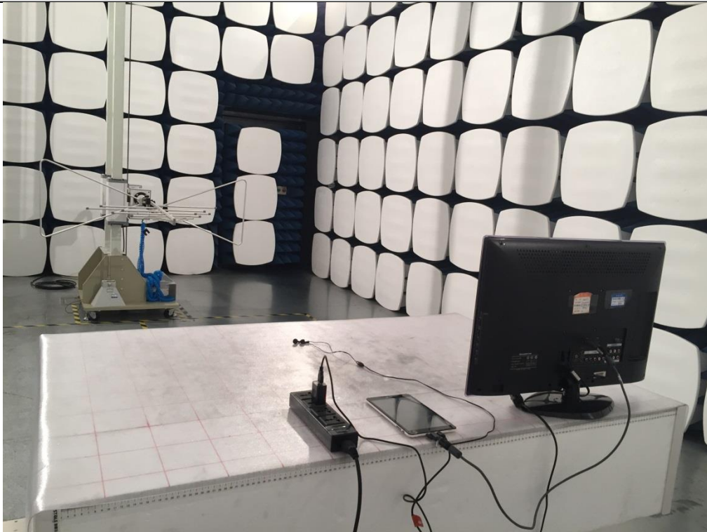
Test setup photo for HDMI mode Radiated Emission
