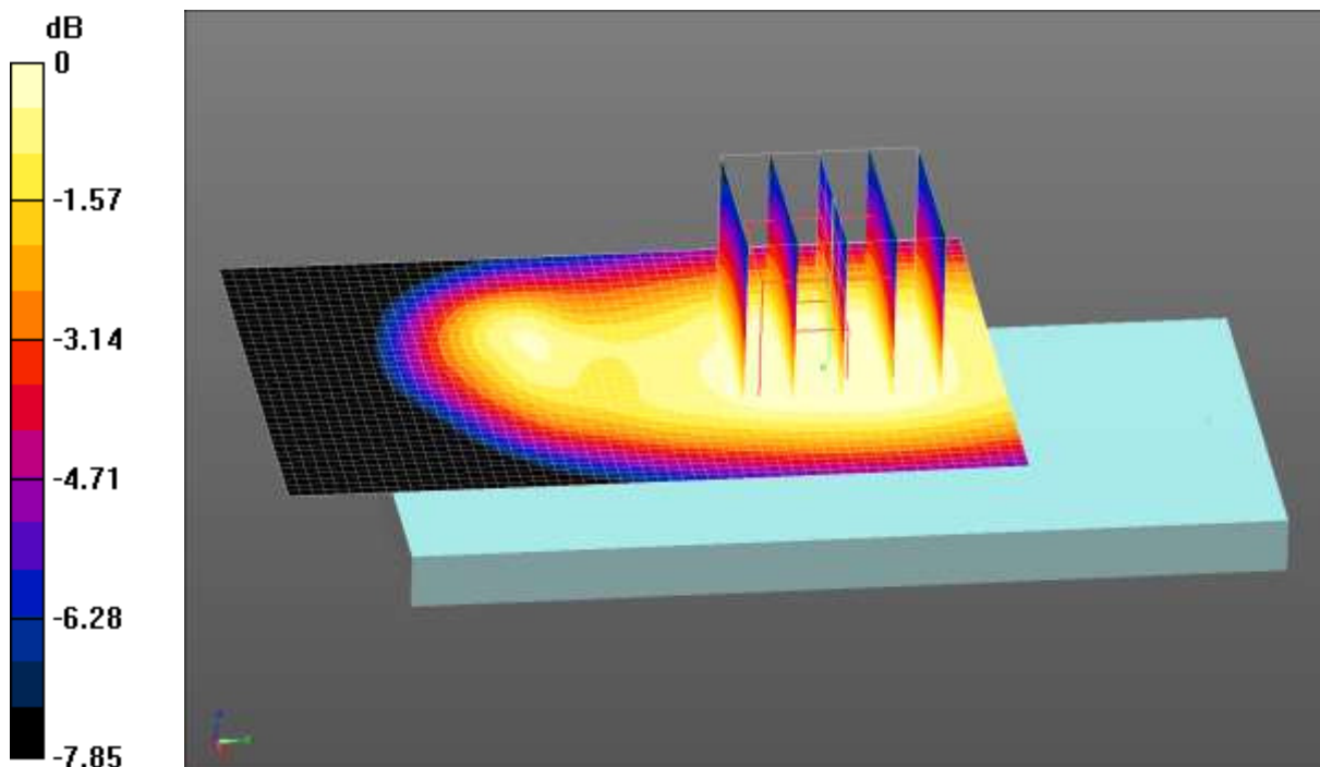
0 dB = 0.457 W/kg = -3.40 dBW/kg
