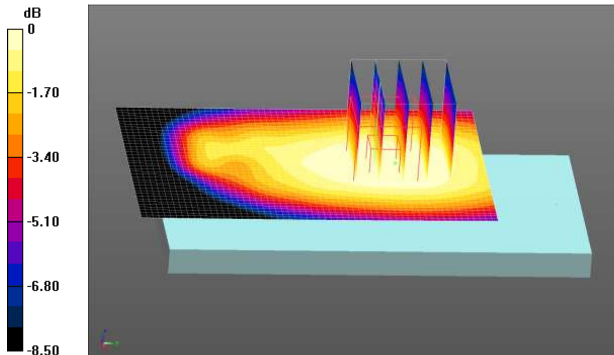
0 dB = 0.400 W/kg = -3.98 dBW/kg
