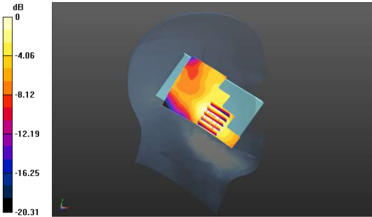
0 dB = 0.236 \text{ W/kg} = -6.27 \text{ dBW/kg}
