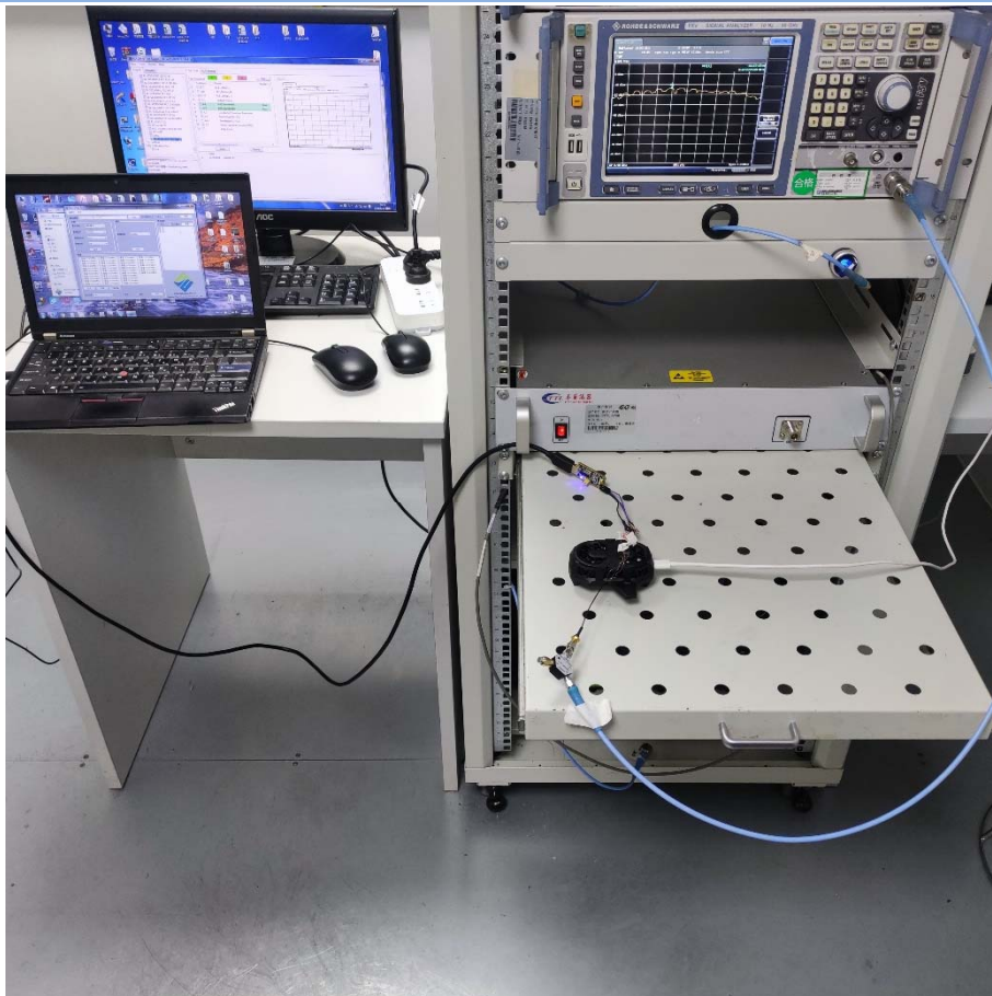
Conducted Test
