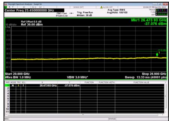
n41(80M)_DFT-s-OFDM_BPSK_ Edge_1RB_Left_Low_CH
