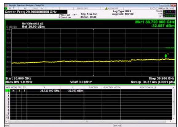
n77(100M)_DFT-s-OFDM_BPSK_ Edge_1RB_Left_High_CH
