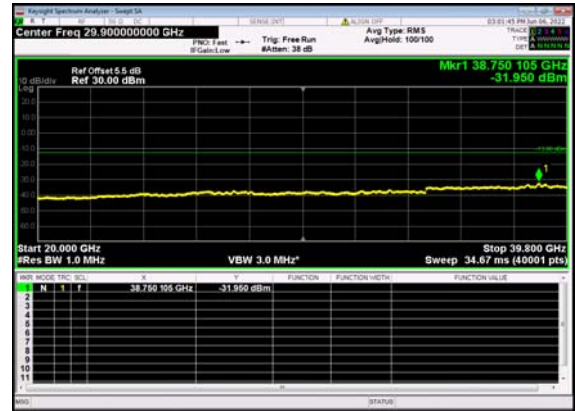
n77(30M)_DFT-s-OFDM_QPSK_ Edge_1RB_Left_High_CH
