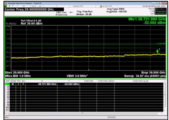
n77(40M)_DFT-s-OFDM_BPSK_ Edge_1RB_Left_Mid_CH
