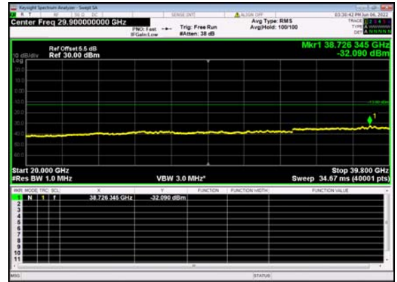
n77(100M)_DFT-s-OFDM_BPSK_ Edge_1RB_Left_Mid_CH
