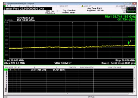
n77(60M)_DFT-s-OFDM_QPSK_ Edge_1RB_Left_Low_CH
