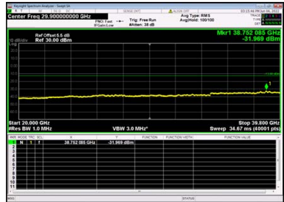
n77(60M)_DFT-s-OFDM_QPSK_ Edge_1RB_Left_Mid_CH
