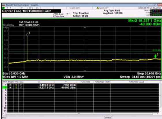
n41(80M)_DFT-s-OFDM_QPSK_ Edge_1RB_Left_Low_CH
