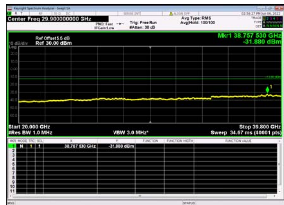
n77(30M)_DFT-s-OFDM_QPSK_ Edge_1RB_Left_Low_CH
