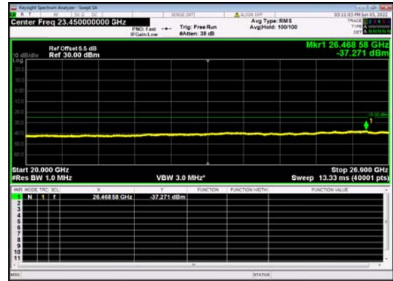
n41(80M)_DFT-s-OFDM_QPSK_ Edge_1RB_Left_High_CH
