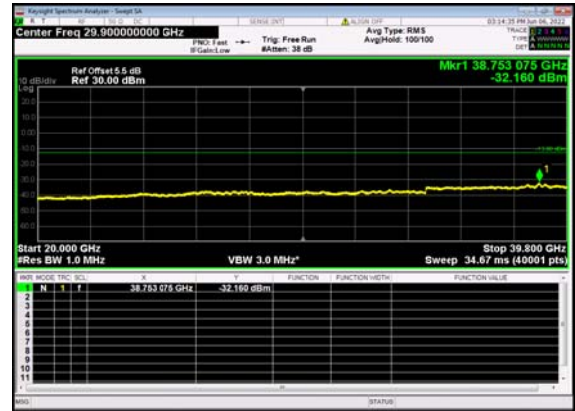
n77(60M)_DFT-s-OFDM_BPSK_ Edge_1RB_Left_Mid_CH
