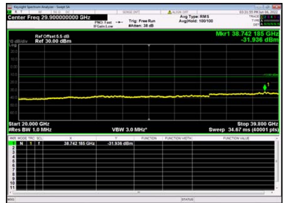
n77(100M)_DFT-s-OFDM_QPSK_ Edge_1RB_Left_Mid_CH
