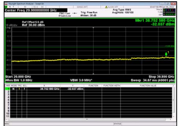
n77(40M)_DFT-s-OFDM_QPSK_ Edge_1RB_Left_Mid_CH
