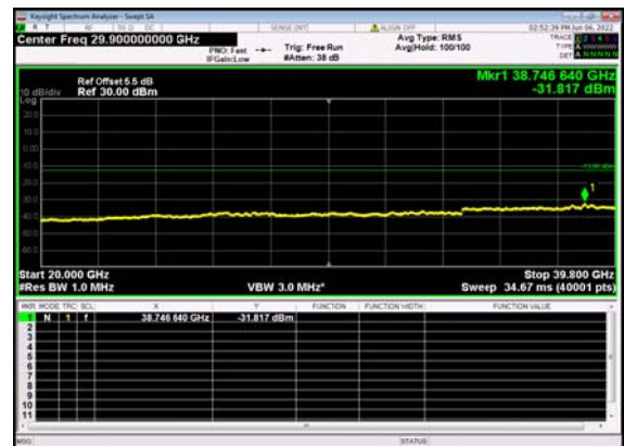
n77(20M)_DFT-s-OFDM_BPSK_ Edge_1RB_Left_High_CH
