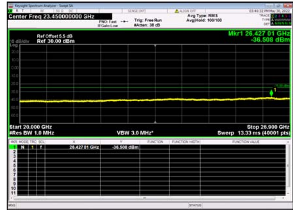
n41(50M)_DFT-s-OFDM_QPSK_ Edge_1RB_Left_High_CH
