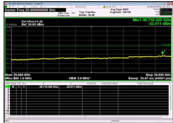
n77(30M)_DFT-s-OFDM_QPSK_ Edge_1RB_Left_Mid_CH
