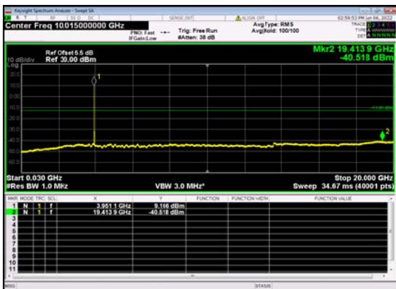
n77(30M)_DFT-s-OFDM_BPSK_ Edge_1RB_Left_High_CH
