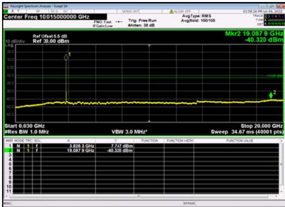
n77(30M)_DFT-s-OFDM_QPSK_ Edge_1RB_Left_Mid_CH
