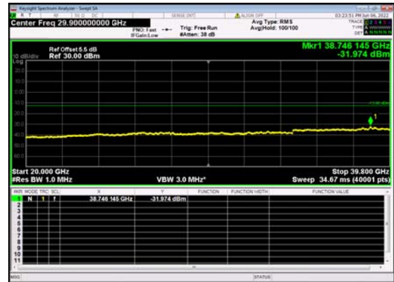
n77(80M)_DFT-s-OFDM_QPSK_ Edge_1RB_Left_Mid_CH
