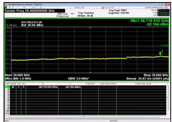
n77(40M)_DFT-s-OFDM_BPSK_ Edge_1RB_Left_High_CH
