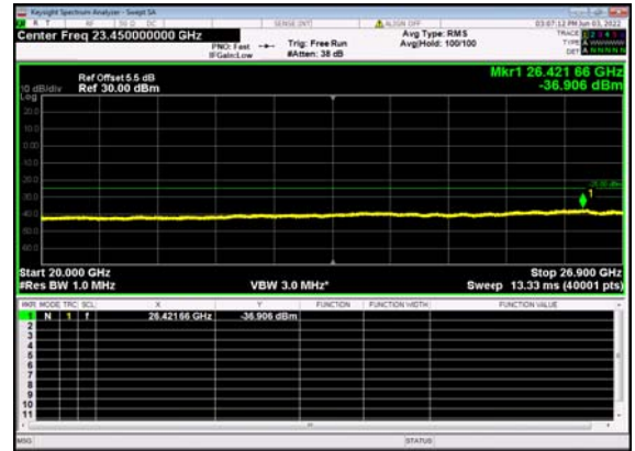
n41(80M)_DFT-s-OFDM_BPSK_ Edge_1RB_Left_Mid_CH
