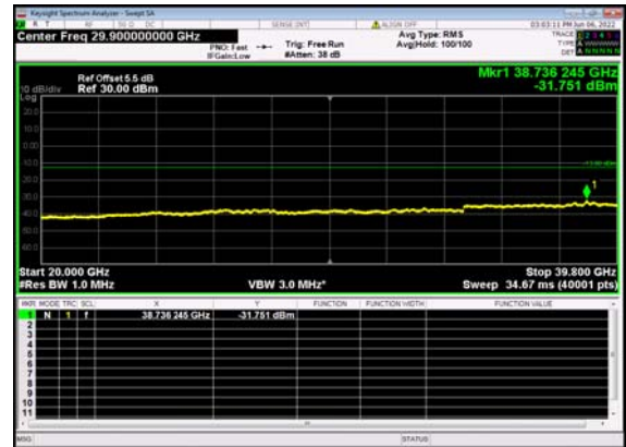
n77(40M)_DFT-s-OFDM_BPSK_ Edge_1RB_Left_Low_CH
