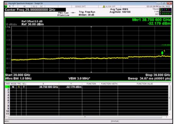
n77(40M)_DFT-s-OFDM_QPSK_ Edge_1RB_Left_High_CH
