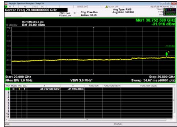
n77(30M)_DFT-s-OFDM_BPSK_ Edge_1RB_Left_Mid_CH
