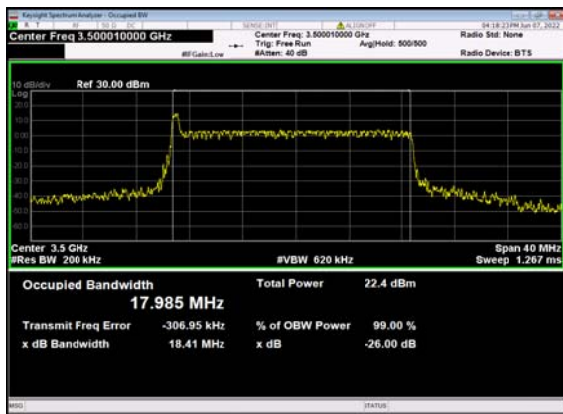
n77(20M)_DFT-s-OFDM_PI_2-BPSK_ Outer_Full_633334_CH
