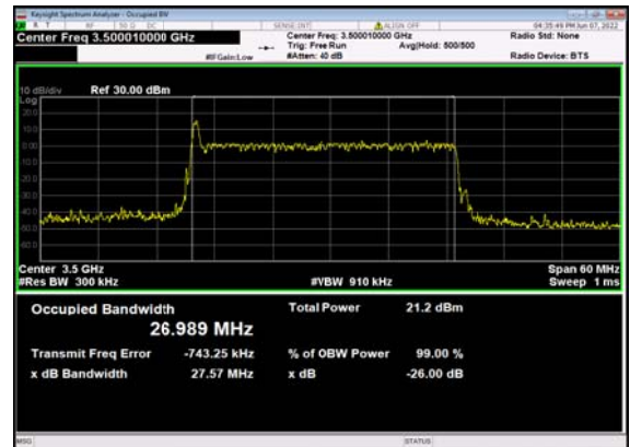
n77(30M)_DFT-s-OFDM_64 QAM_Outer_Full_633334_CH
