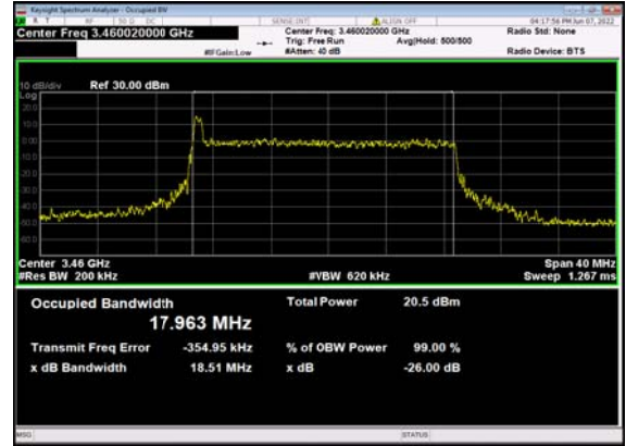
n77(20M)_CP-OFDM_QPSK_ Outer_Full_630668_CH
