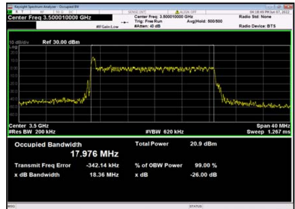
n77(20M)_DFT-s-OFDM_64 QAM_Outer_Full_633334_CH
