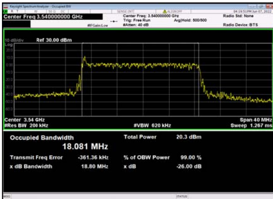
n77(20M)_DFT-s-OFDM_16 QAM_Outer_Full_636000_CH
