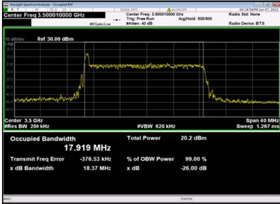
n77(20M)_DFT-s-OFDM_256 QAM_Outer_Full_633334_CH
