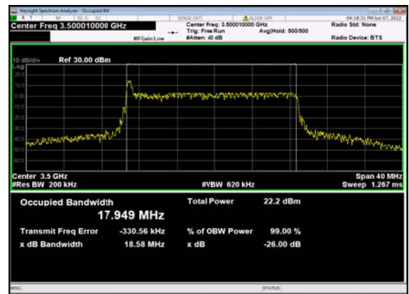
n77(20M)_DFT-s-OFDM_QPSK_ Outer_Full_633334_CH
