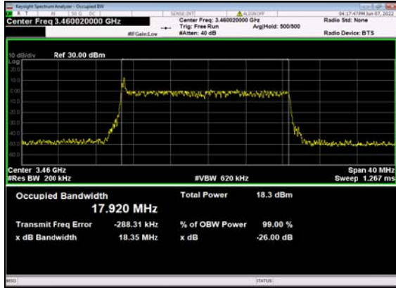
n77(20M)_DFT-s-OFDM_256 QAM_Outer_Full_630668_CH
