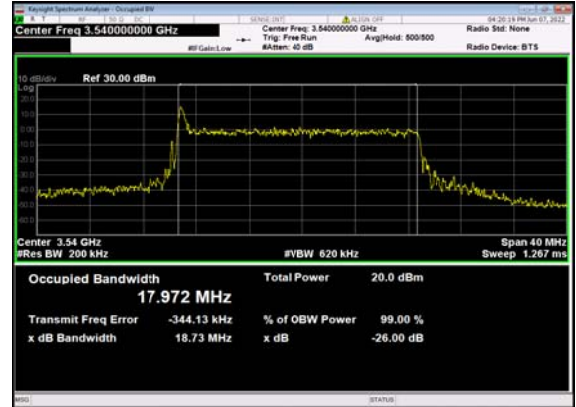
n77(20M)_CP-OFDM_QPSK_ Outer_Full_636000_CH
