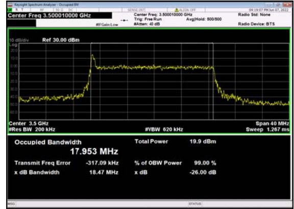
n77(20M)_CP-OFDM_QPSK_ Outer_Full_633334_CH
