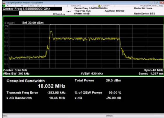
n77(20M)_DFT-s-OFDM_256 QAM_Outer_Full_636000_CH
