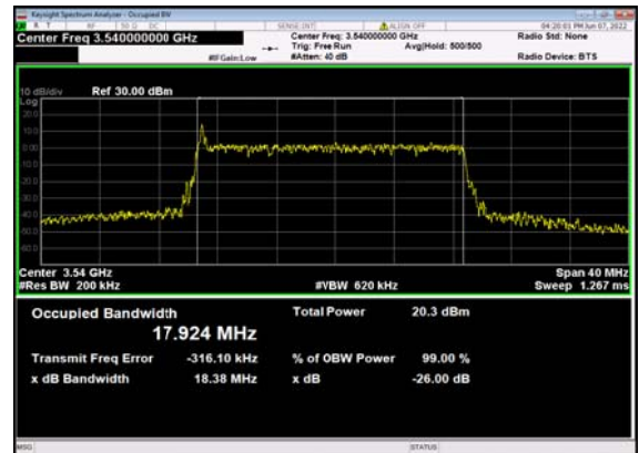
n77(20M)_DFT-s-OFDM_64 QAM_Outer_Full_636000_CH
