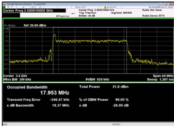
n77(20M)_DFT-s-OFDM_16 QAM_Outer_Full_633334_CH
