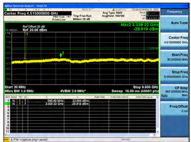
B5 / 3MHz / High CH / 64QAM
