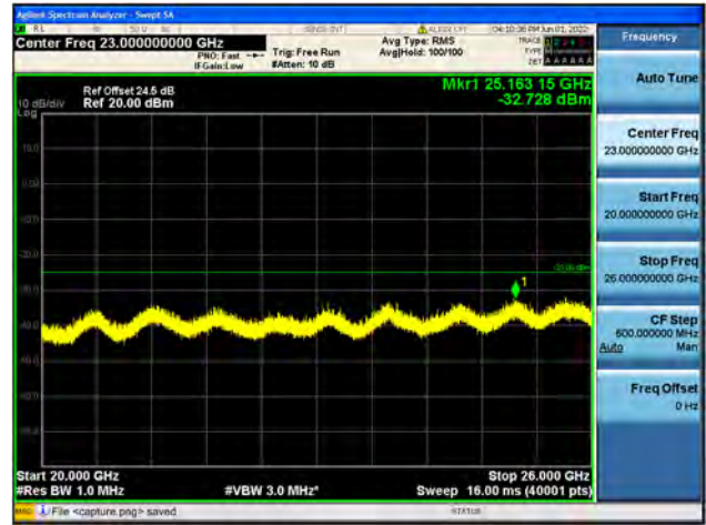
B7-20G-26G / 20MHz / Mid CH / 16QAM
