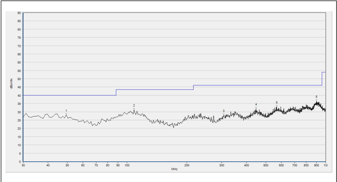
(30MHz – 1GHz, Test Antenna Horizontal)
