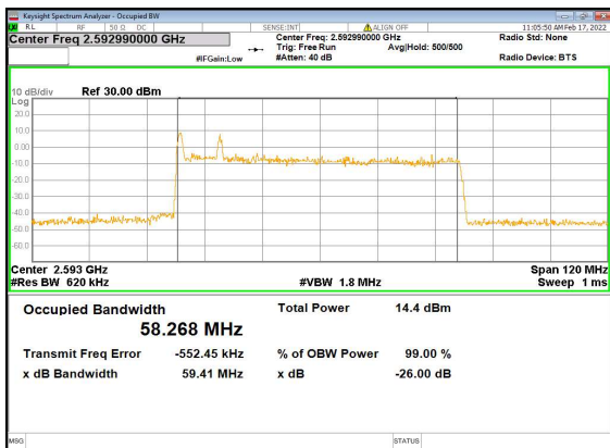
B2_n41(60M)_DFT-s-OFDM_16QAM_Outer_Full_Mid_CH
