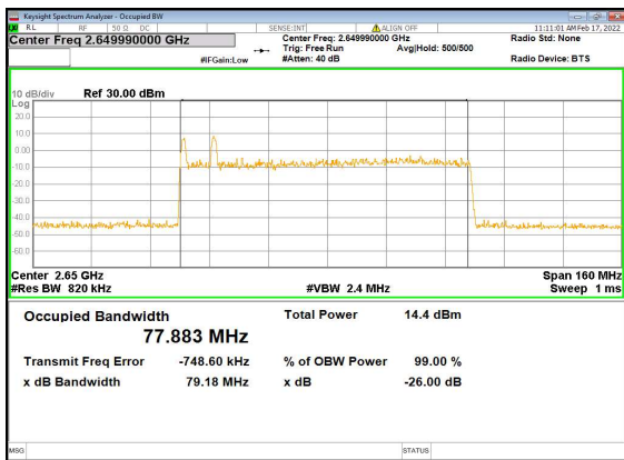
B2_n41(80M)_DFT-s-OFDM_16QAM_Outer_Full_High_CH
