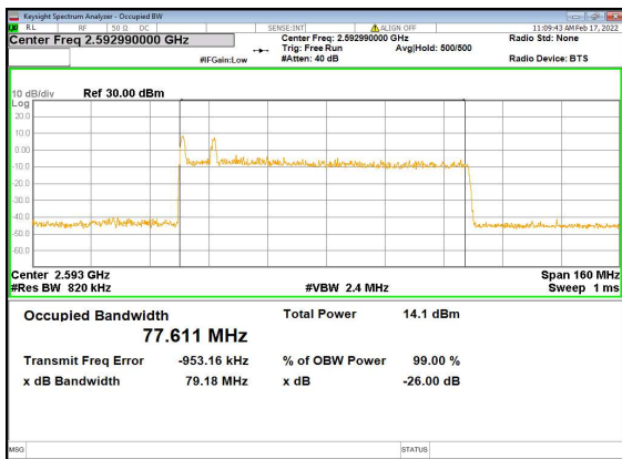
B2_n41(80M)_DFT-s-OFDM_16QAM_Outer_Full_Mid_CH
