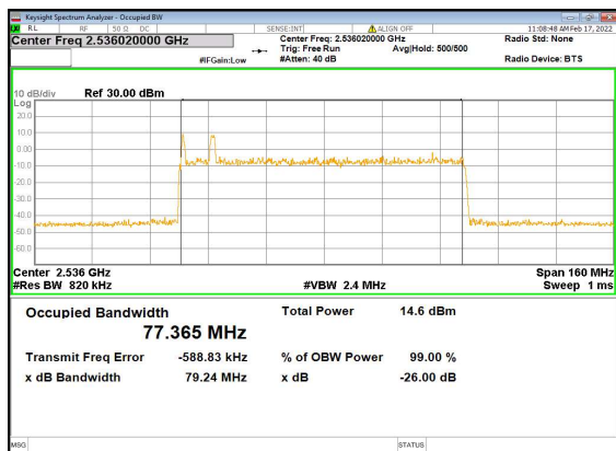
B2_n41(80M)_DFT-s-OFDM_256QAM_Outer_Full_Low_CH
