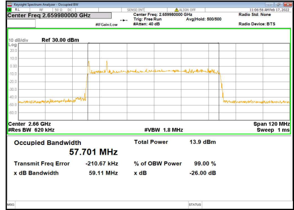
B2_n41(60M)_DFT-s-OFDM_QPSK_Outer_Full_High_CH
