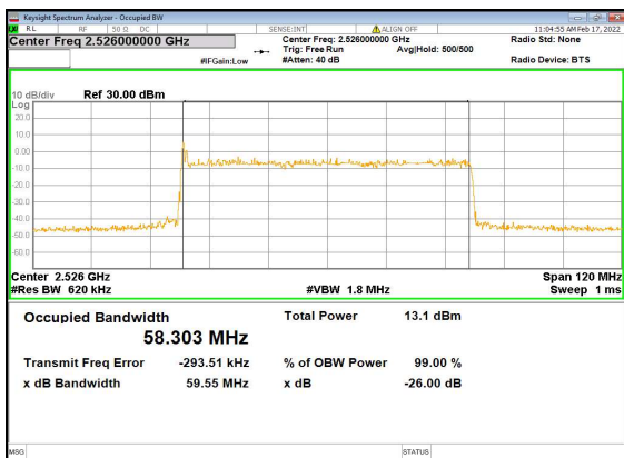
B2_n41(60M)_DFT-s-OFDM_256QAM_Outer_Full_Low_CH
