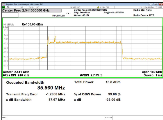
B2_n41(90M)_DFT-s-OFDM_16QAM_Outer_Full_Low_CH
