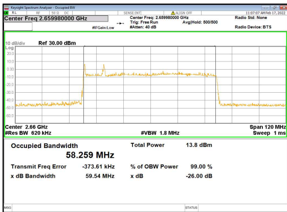
B2_n41(60M)_DFT-s-OFDM_16QAM_Outer_Full_High_CH
