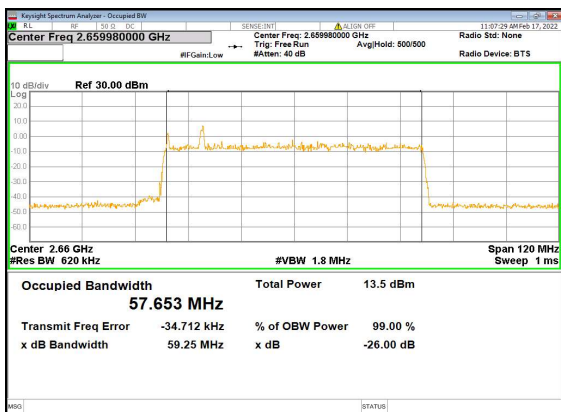
B2_n41(60M)_DFT-s-OFDM_256QAM_Outer_Full_High_CH
