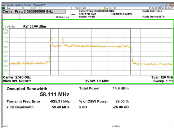
B2_n41(60M)_DFT-s-OFDM_256QAM_Outer_Full_Mid_CH
