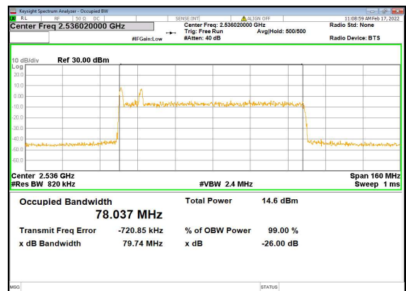
B2_n41(80M)_CP-OFDM_QPSK_Outer_Full_Low_CH
