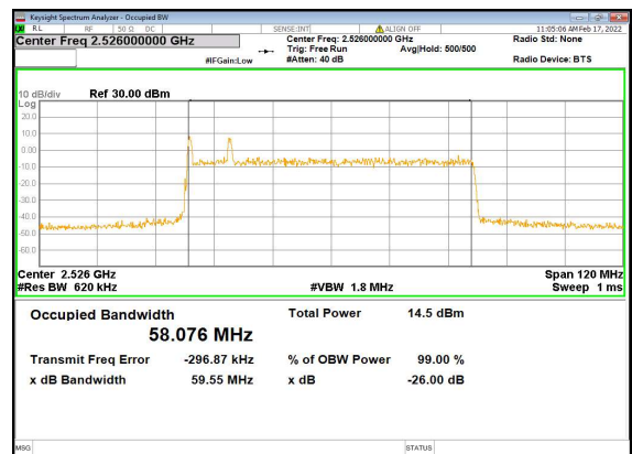
B2_n41(60M)_CP-OFDM_QPSK_Outer_Full_Low_CH
