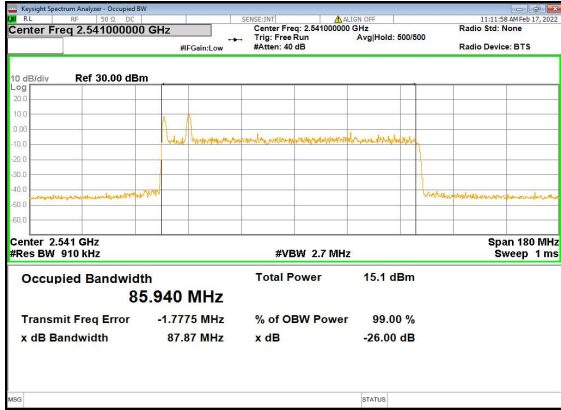
B2_n41(90M)_DFT-s-OFDM_PI_2-BPSK_Outer_Full_Low_CH
