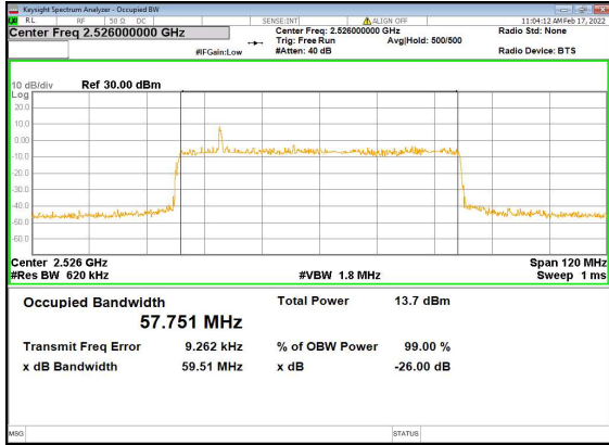
B2_n41(60M)_DFT-s-OFDM_PI_2-BPSK_Outer_Full_Low_CH
