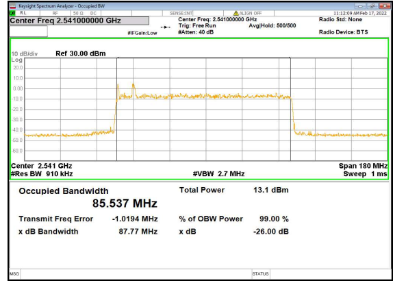
B2_n41(90M)_DFT-s-OFDM_QPSK_Outer_Full_Low_CH
