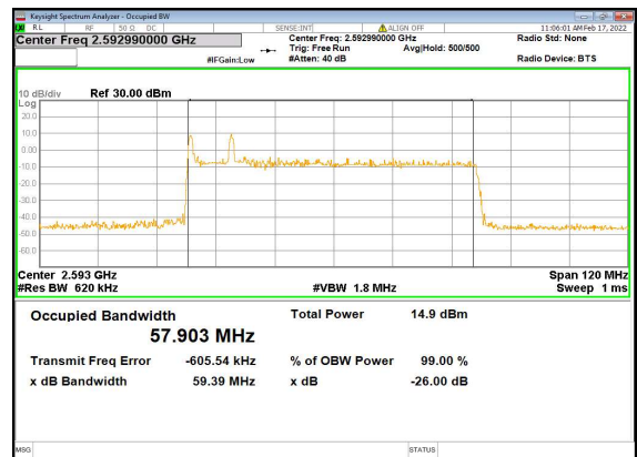
B2_n41(60M)_DFT-s-OFDM_64QAM_Outer_Full_Mid_CH
