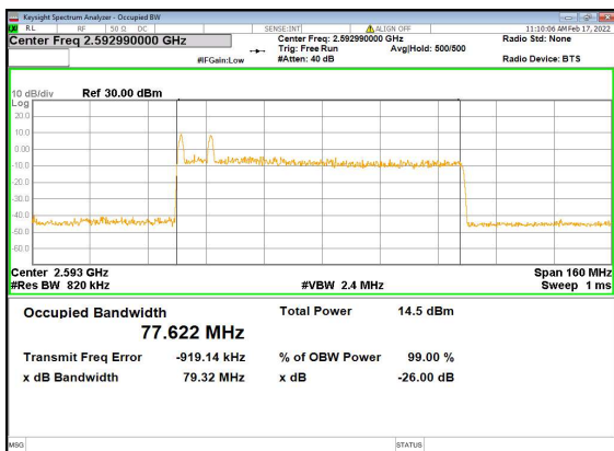
B2_n41(80M)_DFT-s-OFDM_256QAM_Outer_Full_Mid_CH
