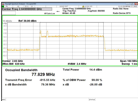
B2_n41(80M)_DFT-s-OFDM_256QAM_Outer_Full_High_CH
