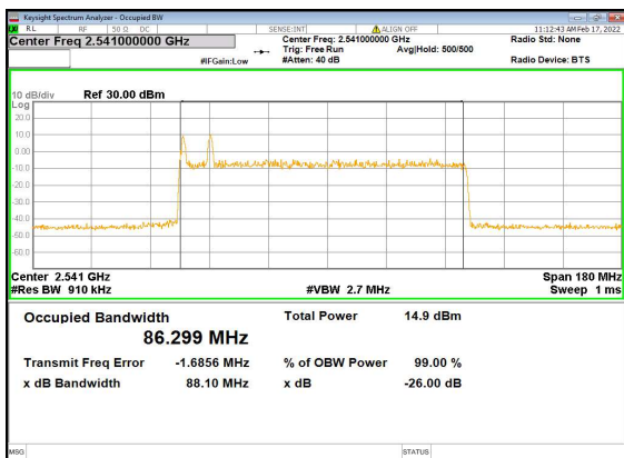
B2_n41(90M)_DFT-s-OFDM_256QAM_Outer_Full_Low_CH
