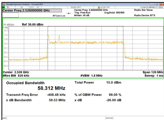
B2_n41(60M)_DFT-s-OFDM_16QAM_Outer_Full_Low_CH
