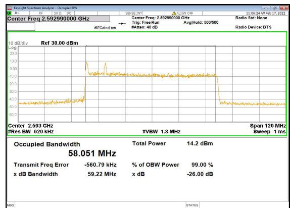
B2_n41(60M)_CP-OFDM_QPSK_Outer_Full_Mid_CH
