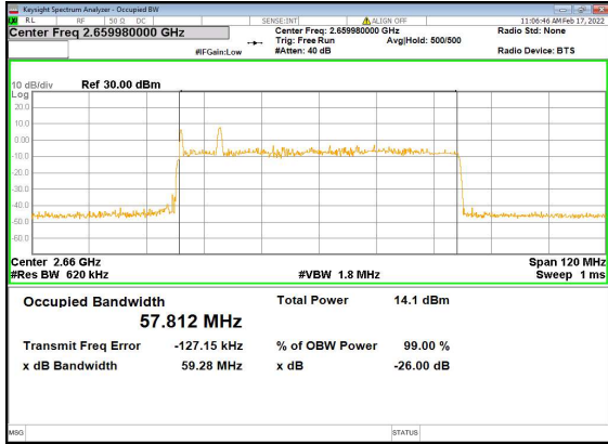
B2_n41(60M)_DFT-s-OFDM_PI_2-BPSK_Outer_Full_High_CH
