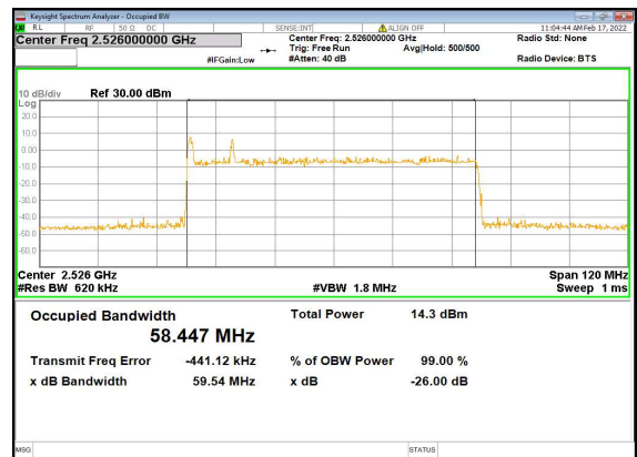
B2_n41(60M)_DFT-s-OFDM_64QAM_Outer_Full_Low_CH
