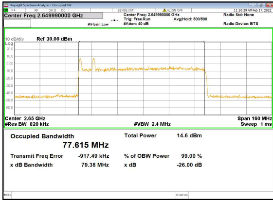
B2_n41(80M)_DFT-s-OFDM_PI_2-BPSK_Outer_Full_High_CH
