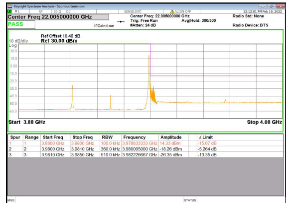
n77(60M)_DFT-s-OFDM_QPSK_Edge_1RB_ Right_High_CH
