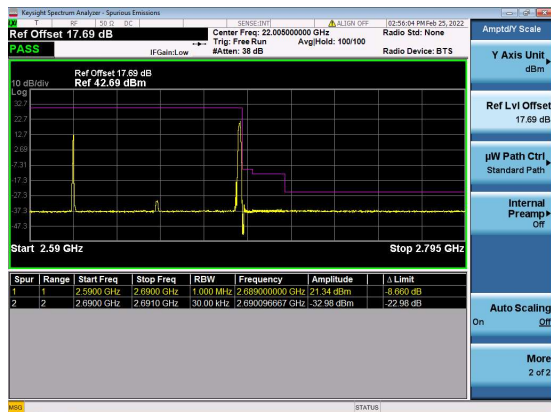
n41(80M)_DFT-s-OFDM_BPSK_Edge_1RB_ Right_High_CH
