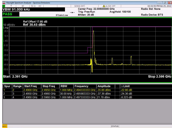
n41(50M)_DFT-s-OFDM_BPSK_Edge_1RB_ Left_Low_CH
