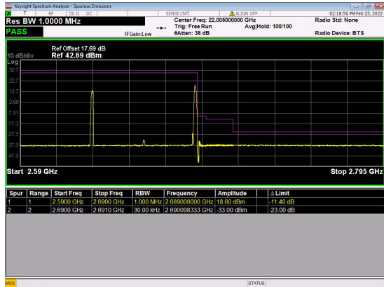
n41(60M)_DFT-s-OFDM_BPSK_Edge_1RB_ Right_High_CH
