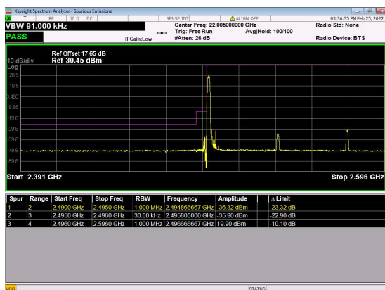
n41(80M)_DFT-s-OFDM_BPSK_Edge_1RB_ Left_Low_CH
