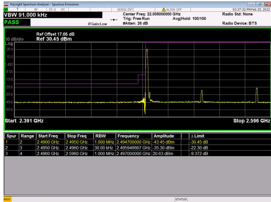
n41(90M)_DFT-s-OFDM_BPSK_Edge_1RB_ Left_Low_CH
