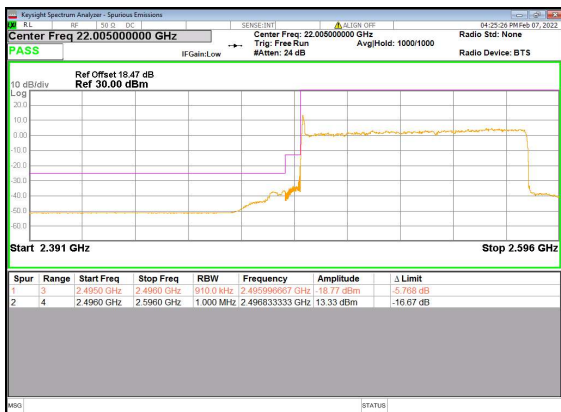
n41(90M)_DFT-s-OFDM_BPSK_Outer_Full_ Low_CH
