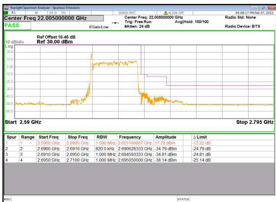
n41(40M)_DFT-s-OFDM_BPSK_Outer_Full_ High_CH
