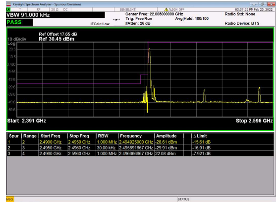
n41(90M)_DFT-s-OFDM_QPSK_Edge_1RB_ Left_Low_CH
