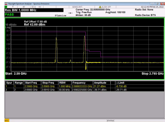
n41(40M)_DFT-s-OFDM_QPSK_Edge_1RB_ Right_High_CH
