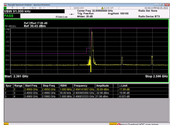
n41(80M)_DFT-s-OFDM_QPSK_Edge_1RB_ Left_Low_CH
