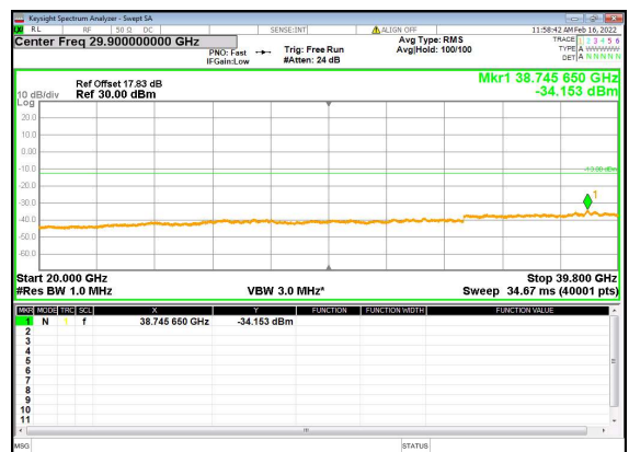
n77(30M)_DFT-s-OFDM_BPSK_Edge_1RB_ Left_Mid_CH
