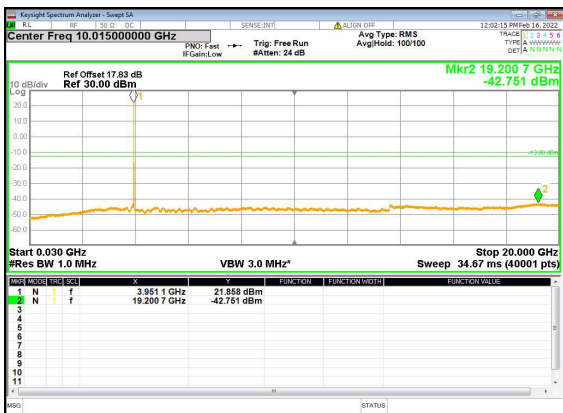
n77(30M)_DFT-s-OFDM_QPSK_Edge_1RB_ Left_High_CH
