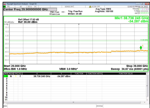
n77(30M)_DFT-s-OFDM_QPSK_Edge_1RB_ Left_High_CH
