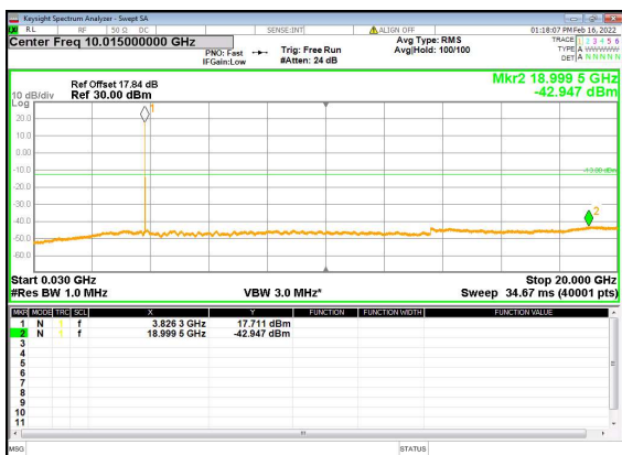
n77(30M)_DFT-s-OFDM_BPSK_Edge_1RB_ Left_Mid_CH
