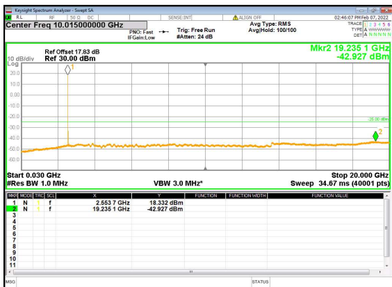
n41(80M)_DFT-s-OFDM_BPSK_Edge_1RB_ Left_Mid_CH
