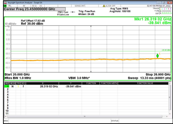
n41(80M)_DFT-s-OFDM_BPSK_Edge_1RB_ Left_High_CH
