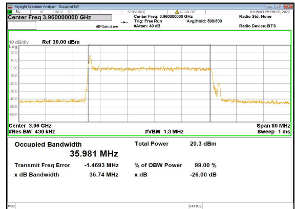
n77(40M)_CP-OFDM_QPSK_Outer_Full_High_CH
