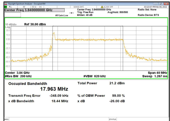
n77(20M)_CP-OFDM_QPSK_Outer_Full_Mid_CH
