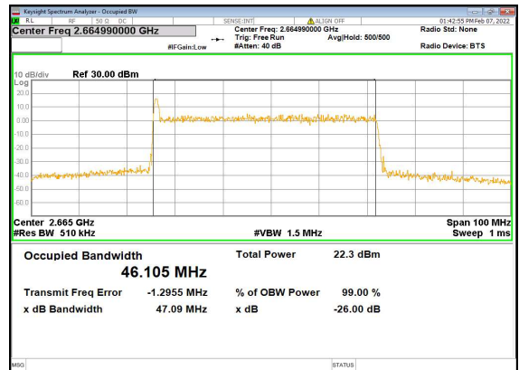
n41(50M)_CP-OFDM_QPSK_Outer_Full_High_CH
