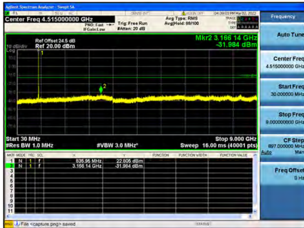
Band19 / 10MHz / High CH / 64QAM
