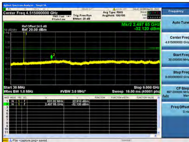
Band19 / 15MHz / Mid CH / 64QAM
