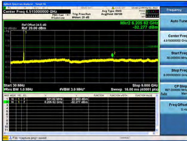
Band19 / 15MHz / Mid CH / QPSK
