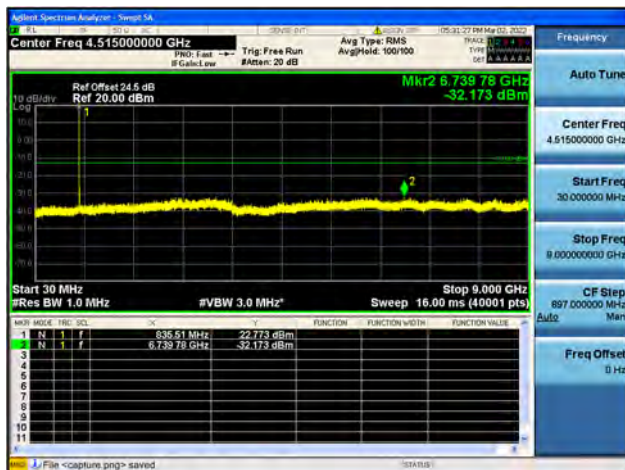
Band19 / 5MHz / Mid CH / 64QAM
