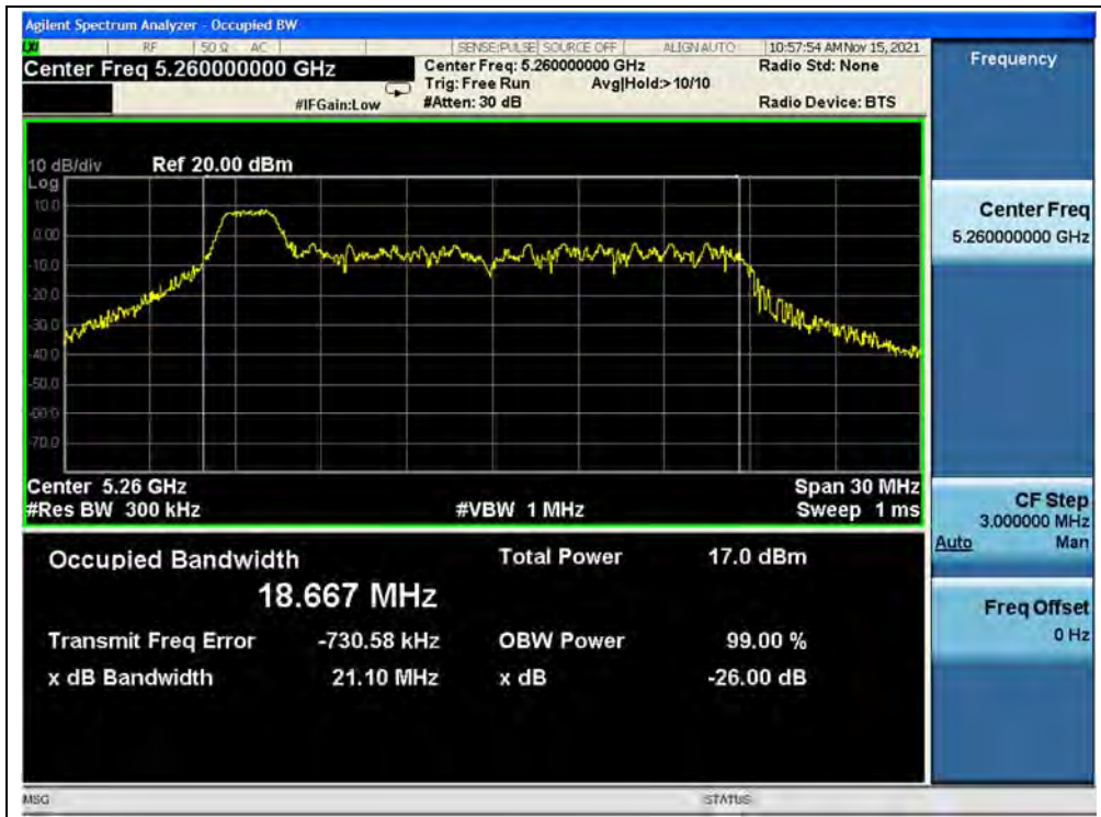
(Channel 52, 5260MHz, 802.11ax (HEW20) RU26)
