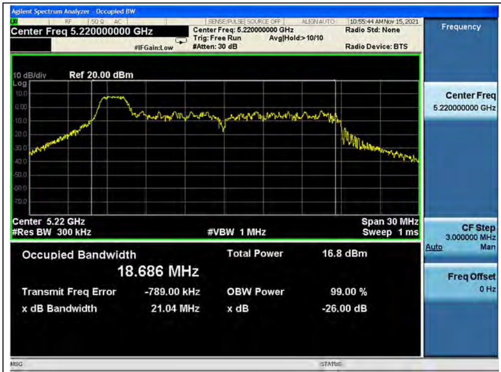
(Channel 44, 5220MHz, 802.11ax (HEW20) RU26)
