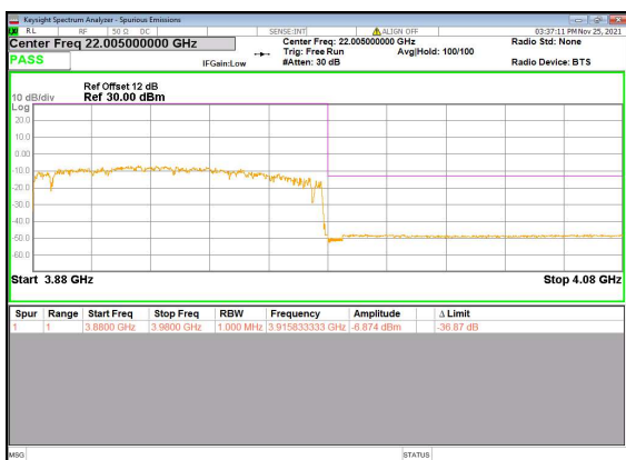
N77(100M)_DFT-s-OFDM_BPSK_Outer_Full_High_CH
