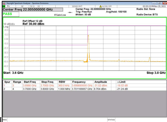
N77(80M)_DFT-s-OFDM_BPSK_Edge_1RB_Left_Low
