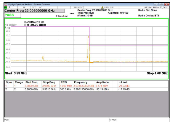
N77(60M)_DFT-s-OFDM_QPSK_Edge_1RB_Right_Hig
