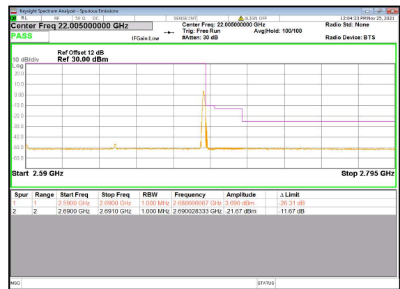
N41(100M)_DFT-s-OFDM_QPSK_Outer_Full_High_CH
