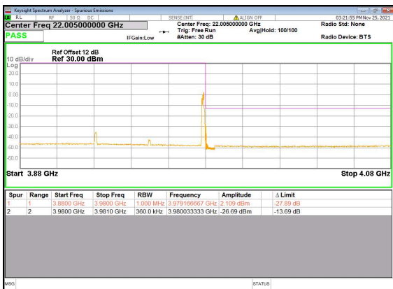
N77(60M)_DFT-s-OFDM_BPSK_Edge_1RB_Right_Hig
