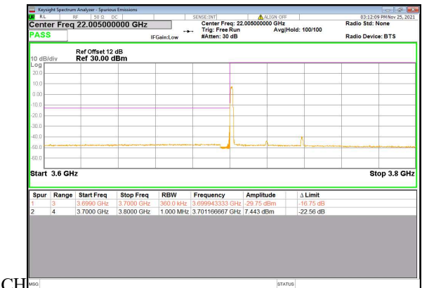
N77(40M)_DFT-s-OFDM_QPSK_Edge_1RB_Left_Low CH
