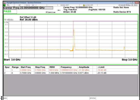
N77(80M)_DFT-s-OFDM_QPSK_Edge_1RB_Left_Low
