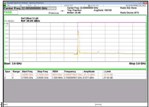
N77(60M)_DFT-s-OFDM_QPSK_Edge_1RB_Left_Low
