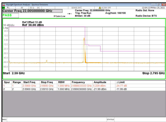
N41(100M)_DFT-s-OFDM_BPSK_Outer_Full_High_CH
