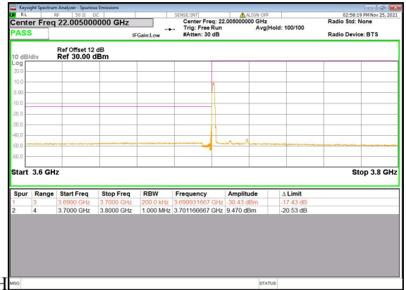
N77(20M)_DFT-s-OFDM_QPSK_Edge_1RB_Left_Low
