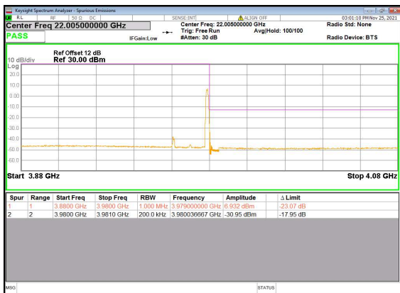
N77(20M)_DFT-s-OFDM_BPSK_Edge_1RB_Right_Hig
