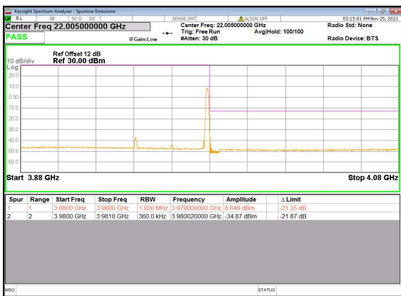
N77(40M)_DFT-s-OFDM_BPSK_Edge_1RB_Right_High_CH
