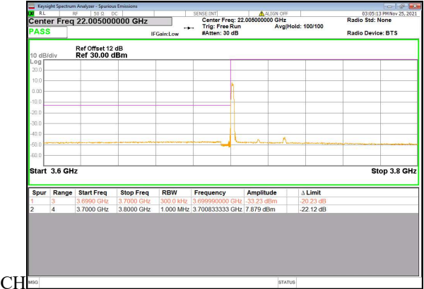
N77(30M)_DFT-s-OFDM_QPSK_Edge_1RB_Left_Low
