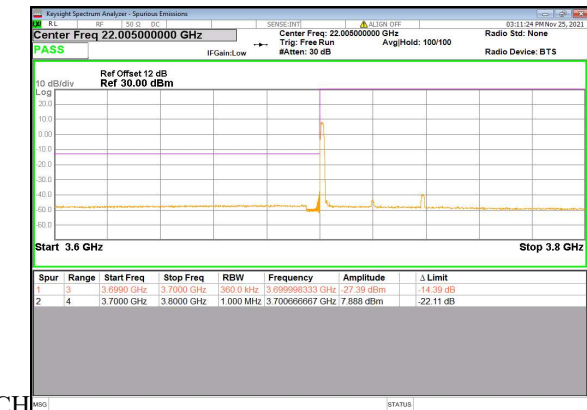
N77(40M)_DFT-s-OFDM_BPSK_Edge_1RB_Left_Low CH
