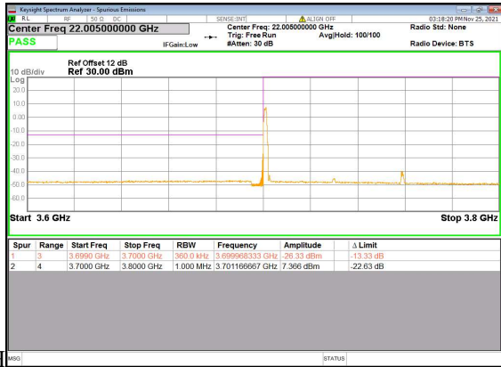
N77(60M)_DFT-s-OFDM_BPSK_Edge_1RB_Left_Low
