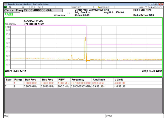
N77(20M)_DFT-s-OFDM_QPSK_Edge_1RB_Right_Hig
