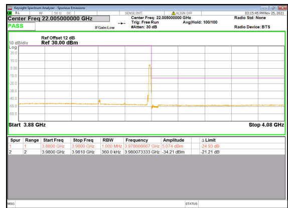
N77(40M)_DFT-s-OFDM_QPSK_Edge_1RB_Right_High_CH
