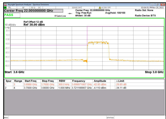
N77(30M)_DFT-s-OFDM_QPSK_Outer_Full_Low_CH
