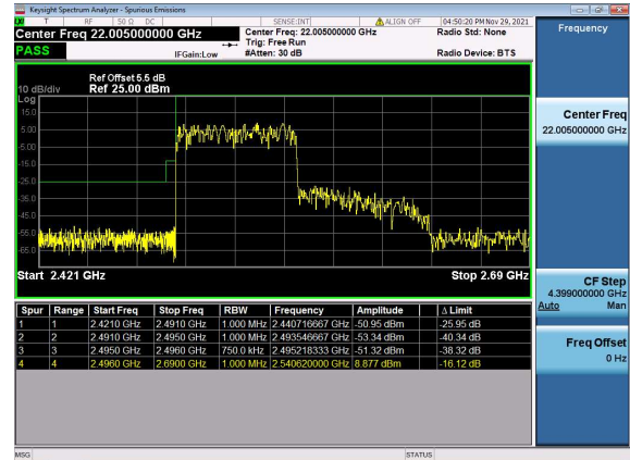
N41(70M)_DFT-s-OFDM_QPSK_Outer_Full_Low_CH
