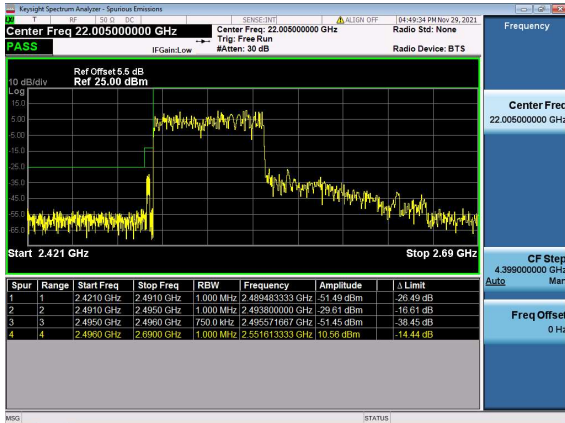
N41(70M)_DFT-s-OFDM_BPSK_Outer_Full_Low_CH
