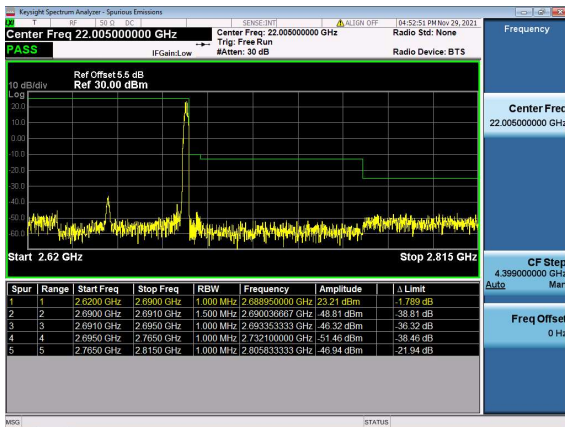
N41(70M)_DFT-s-OFDM_BPSK_Edge_1RB_Right_Hig h_CH
