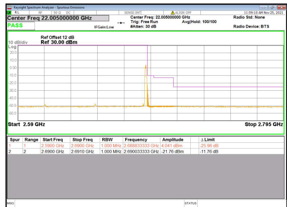
N41(80M)_DFT-s-OFDM_QPSK_Edge_1RB_Right_Hig
