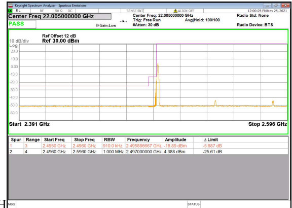
N41(90M)_DFT-s-OFDM_QPSK_Edge_1RB_Left_Low
