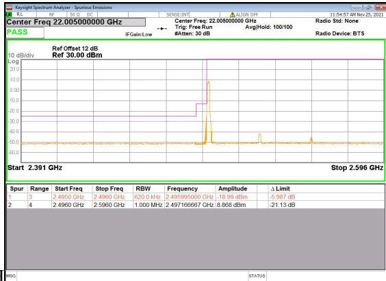
N41(60M)_DFT-s-OFDM_BPSK_Edge_1RB_Left_Low
