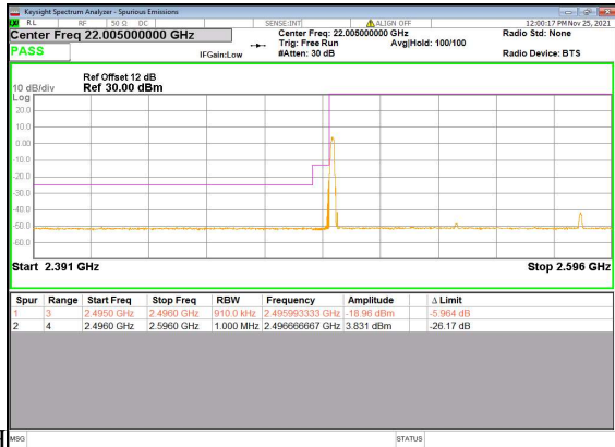
N41(90M)_DFT-s-OFDM_BPSK_Edge_1RB_Left_Low
