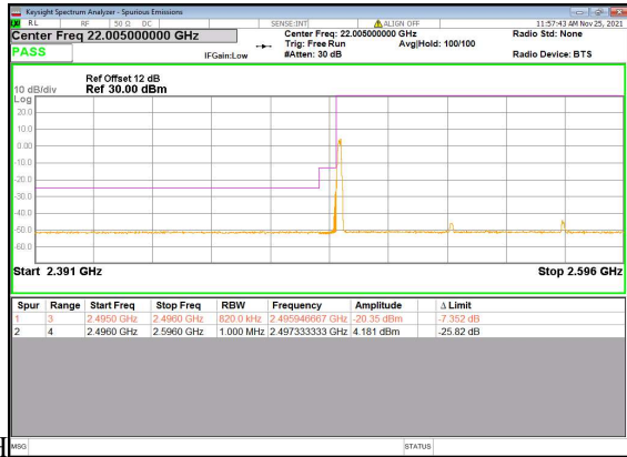
N41(80M)_DFT-s-OFDM_BPSK_Edge_1RB_Left_Low
