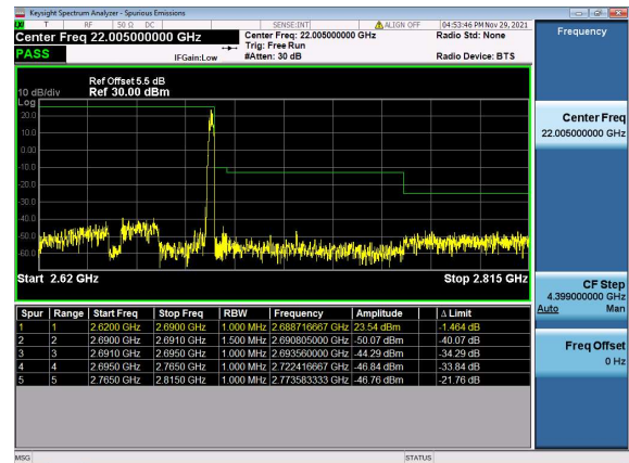
N41(70M)_DFT-s-OFDM_QPSK_Edge_1RB_Right_Hig h_CH
