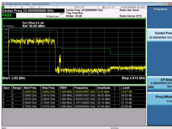
N41(70M)_DFT-s-OFDM_BPSK_Outer_Full_High_CH
