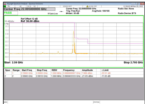
N41(50M)_DFT-s-OFDM_QPSK_Edge_1RB_Right_Hig
