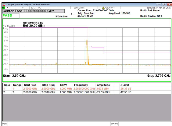
N41(80M)_DFT-s-OFDM_BPSK_Edge_1RB_Right_Hig
