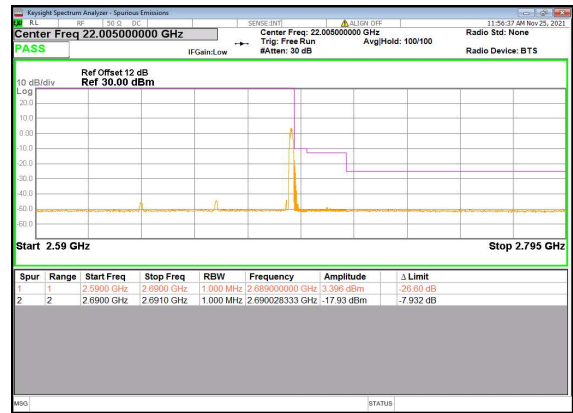
N41(60M)_DFT-s-OFDM_QPSK_Edge_1RB_Right_Hig h_CH
