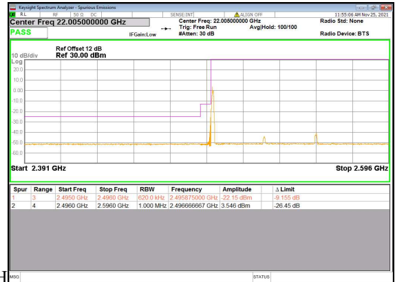
N41(60M)_DFT-s-OFDM_QPSK_Edge_1RB_Left_Low
