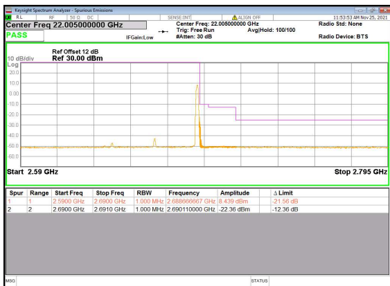
N41(50M)_DFT-s-OFDM_BPSK_Edge_1RB_Right_Hig
