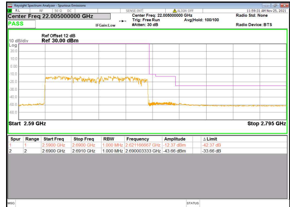
N41(80M)_DFT-s-OFDM_QPSK_Outer_Full_High_CH
