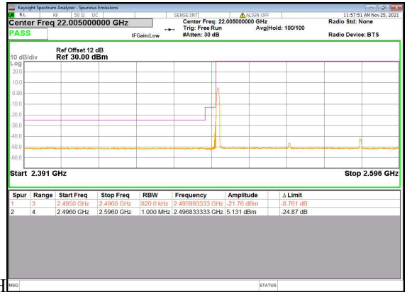
N41(80M)_DFT-s-OFDM_QPSK_Edge_1RB_Left_Low
