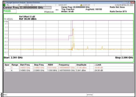
N41(50M)_DFT-s-OFDM_QPSK_Edge_1RB_Left_Low
