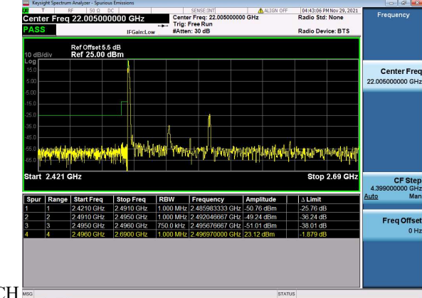
N41(70M)_DFT-s-OFDM_BPSK_Edge_1RB_Left_Low _CH
