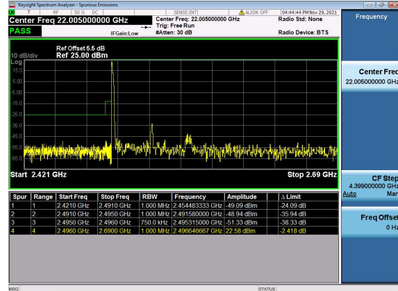
N41(70M)_DFT-s-OFDM_QPSK_Edge_1RB_Left_Low
