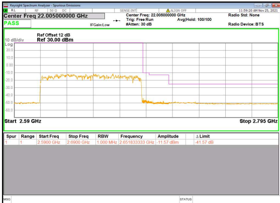
N41(80M)_DFT-s-OFDM_BPSK_Outer_Full_High_CH
