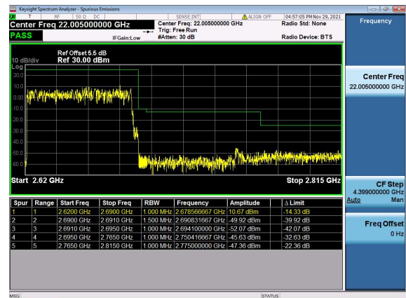
N41(70M)_DFT-s-OFDM_QPSK_Outer_Full_High_CH
