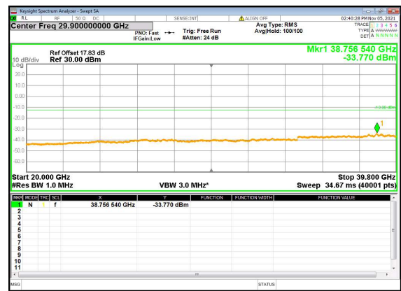
N77(100M)_DFT-s-OFDM_QPSK_Edge_1RB_Left _High_CH
