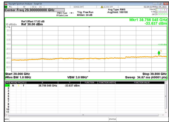
N77(80M)_DFT-s-OFDM_QPSK_Edge_1RB_Left_Mid_CH
