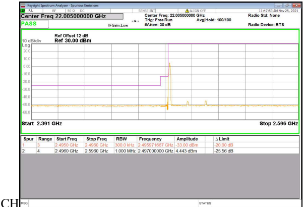
N41(30M)_DFT-s-OFDM_QPSK_Edge_1RB_Left_Low
