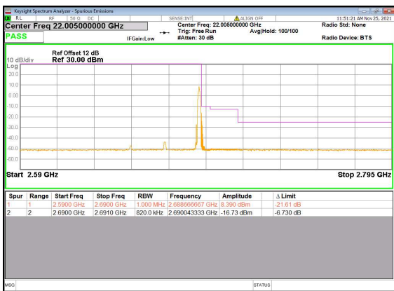
N41(40M)_DFT-s-OFDM_BPSK_Edge_1RB_Right_High_CH
