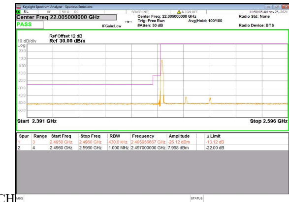
N41(40M)_DFT-s-OFDM_BPSK_Edge_1RB_Left_Low CH
