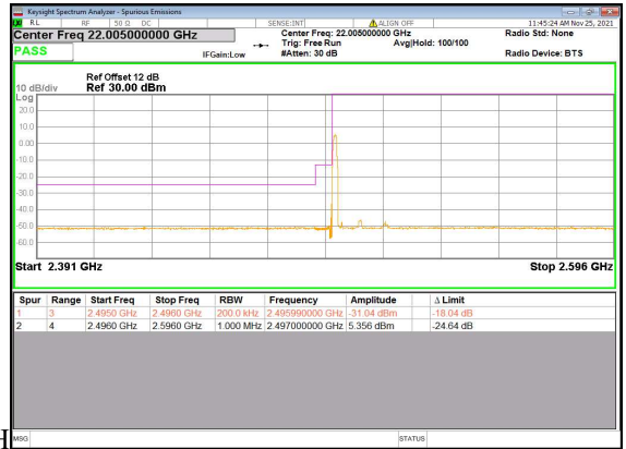
N41(20M)_DFT-s-OFDM_QPSK_Edge_1RB_Left_Low
