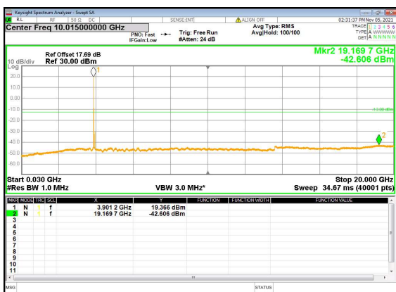
N77(80M)_DFT-s-OFDM_QPSK_Edge_1RB_Left_High_CH
