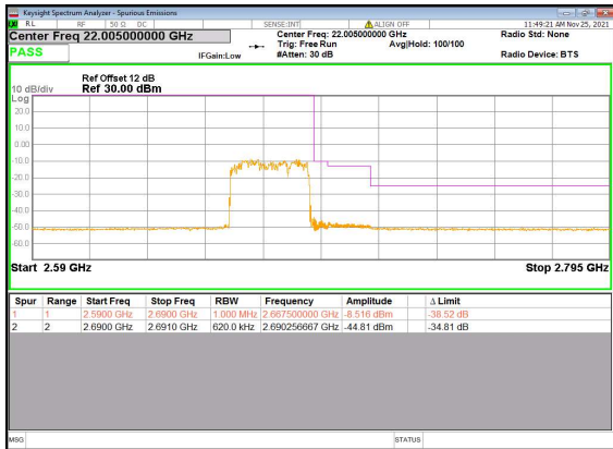
N41(30M)_DFT-s-OFDM_BPSK_Outer_Full_High_CH
