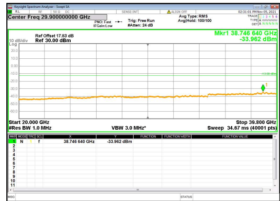
N77(80M)_DFT-s-OFDM_BPSK_Edge_1RB_Left_High_CH
