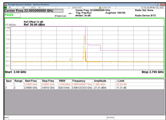
N41(40M)_DFT-s-OFDM_QPSK_Edge_1RB_Right_High_CH
