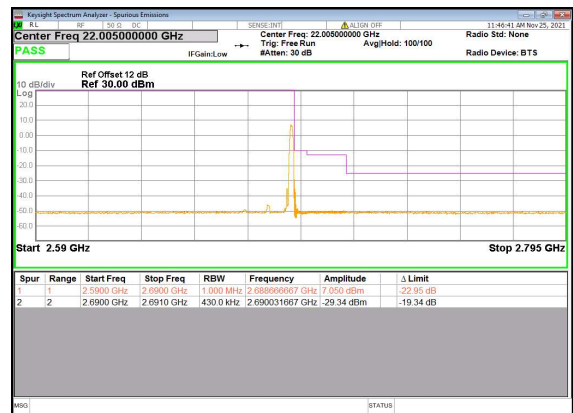
N41(20M)_DFT-s-OFDM_QPSK_Edge_1RB_Right_Hig
