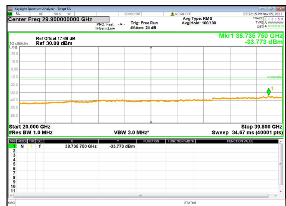
N77(80M)_DFT-s-OFDM_QPSK_Edge_1RB_Left_High_CH
