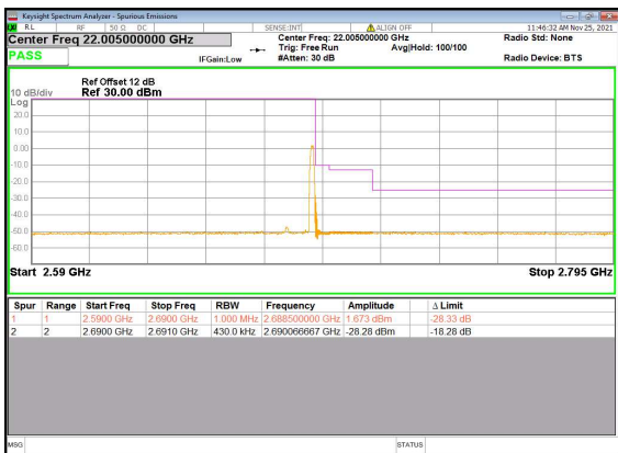
N41(20M)_DFT-s-OFDM_BPSK_Edge_1RB_Right_Hig
