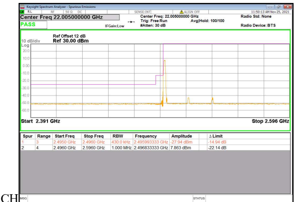
N41(40M)_DFT-s-OFDM_QPSK_Edge_1RB_Left_Low CH
