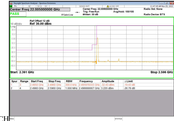
N41(30M)_DFT-s-OFDM_BPSK_Edge_1RB_Left_Low
