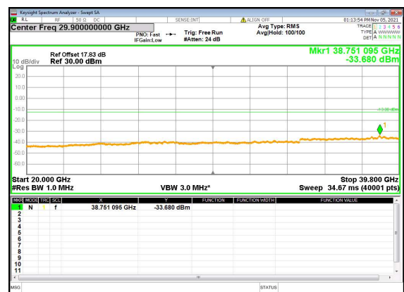
N77(30M)_DFT-s-OFDM_QPSK_Edge_1RB_Left_High_CH
