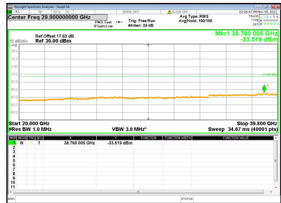
N77(80M)_DFT-s-OFDM_QPSK_Edge_1RB_Left_ Low_CH
