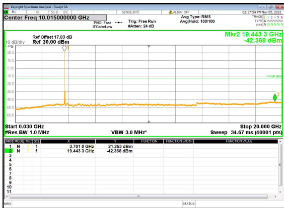
N77(60M)_DFT-s-OFDM_QPSK_Edge_1RB_Left_ Low_CH
