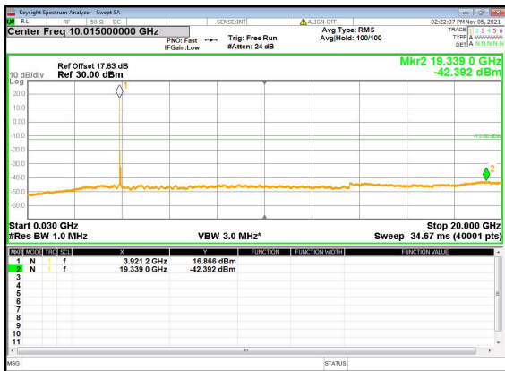
N77(60M)_DFT-s-OFDM_BPSK_Edge_1RB_Left_High_CH
