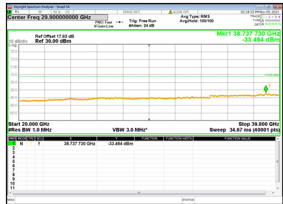
N77(60M)_DFT-s-OFDM_QPSK_Edge_1RB_Left_ Low_CH
