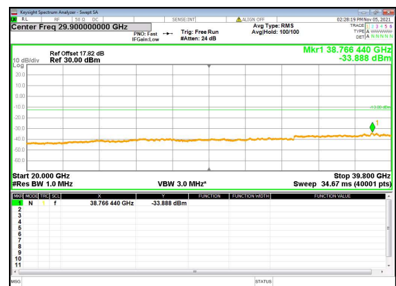
N77(80M)_DFT-s-OFDM_BPSK_Edge_1RB_Left_ Mid_CH
