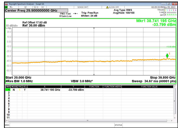
N77(80M)_DFT-s-OFDM_BPSK_Edge_1RB_Left_ Low_CH
