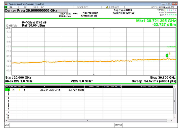
N77(60M)_DFT-s-OFDM_QPSK_Edge_1RB_Left_Mid_CH
