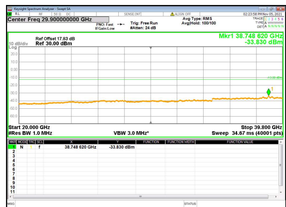
N77(60M)_DFT-s-OFDM_QPSK_Edge_1RB_Left_High_CH
