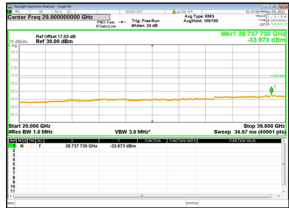
N77(40M)_DFT-s-OFDM_BPSK_Edge_1RB_Left_ Low_CH
