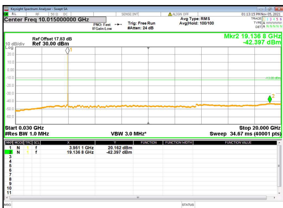
N77(30M)_DFT-s-OFDM_QPSK_Edge_1RB_Left_High_CH
