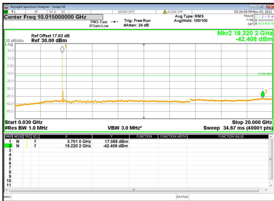
N77(80M)_DFT-s-OFDM_QPSK_Edge_1RB_Left_ Low_CH
