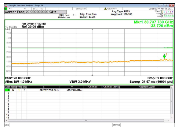
N77(40M)_DFT-s-OFDM_BPSK_Edge_1RB_Left_ Mid_CH
