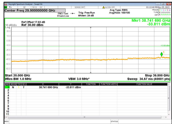
N77(30M)_DFT-s-OFDM_BPSK_Edge_1RB_Left_High_CH
