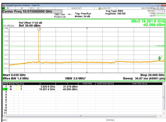
N77(40M)_DFT-s-OFDM_BPSK_Edge_1RB_Left_ Mid_CH
