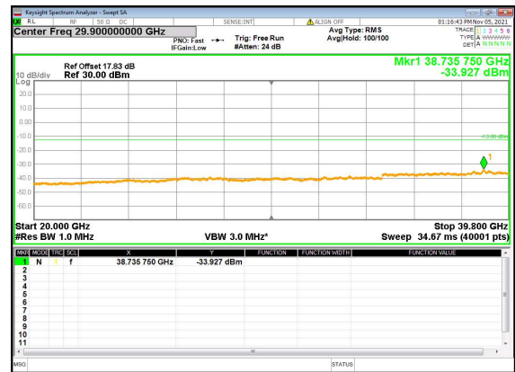
N77(40M)_DFT-s-OFDM_QPSK_Edge_1RB_Left_ Low_CH
