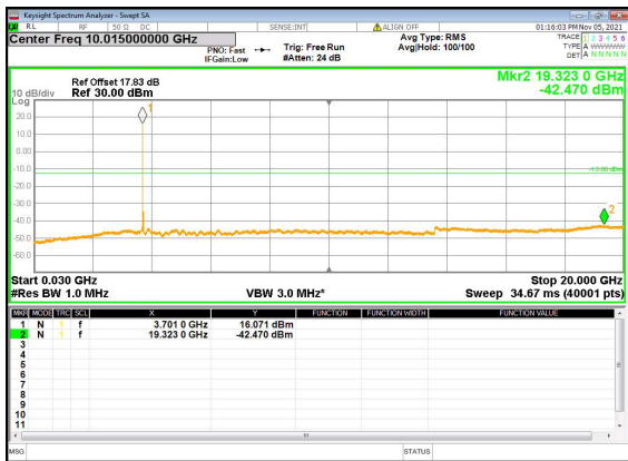
N77(40M)_DFT-s-OFDM_QPSK_Edge_1RB_Left_ Low_CH
