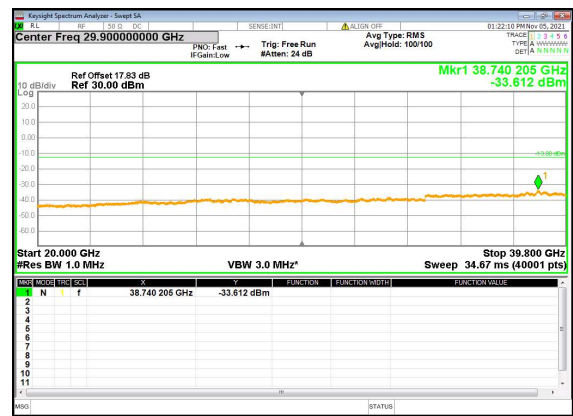
N77(40M)_DFT-s-OFDM_QPSK_Edge_1RB_Left_High_CH
