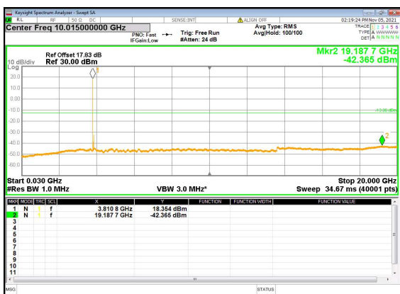
N77(60M)_DFT-s-OFDM_BPSK_Edge_1RB_Left_ Mid_CH
