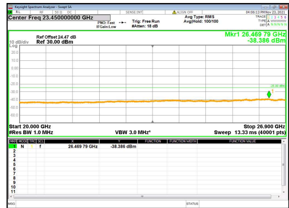
N41(90M)_DFT-s-OFDM_QPSK_Edge_1RB_Left_ Low_CH
