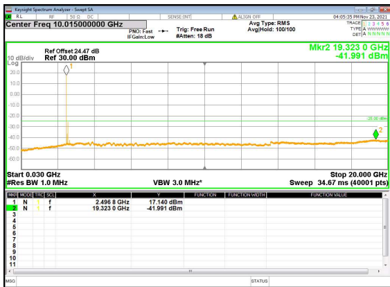
N41(90M)_DFT-s-OFDM_QPSK_Edge_1RB_Left_ Low_CH
