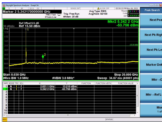
N41(70M)_DFT-s-OFDM_QPSK_Edge_1RB_Left_High_CH
