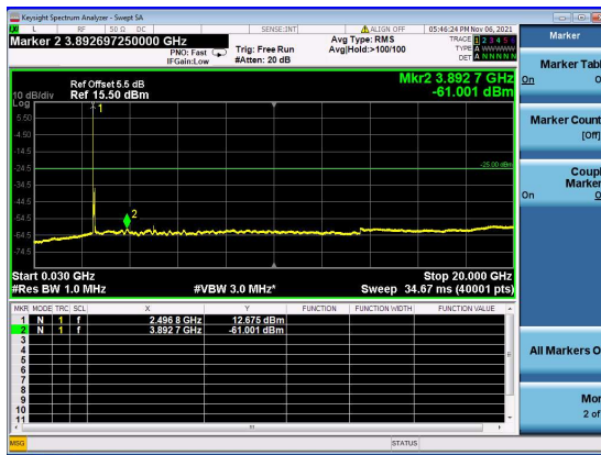
N41(70M)_DFT-s-OFDM_QPSK_Edge_1RB_Left_ Low_CH
