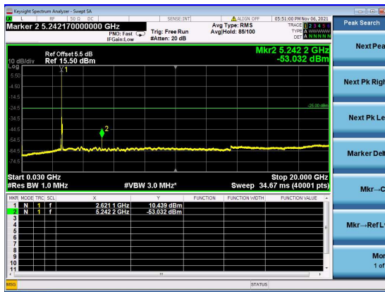
N41(70M)_DFT-s-OFDM_BPSK_Edge_1RB_Left_High_CH
