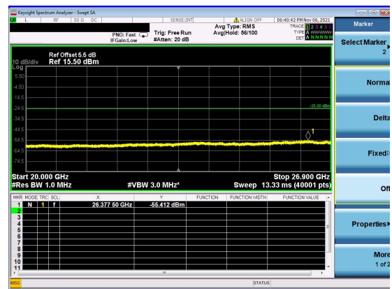
N41(70M)_DFT-s-OFDM_QPSK_Edge_1RB_Left_High_CH
