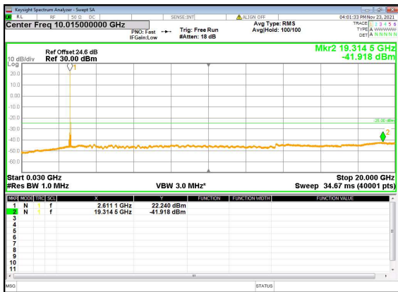
N41(80M)_DFT-s-OFDM_BPSK_Edge_1RB_Left_High_CH
