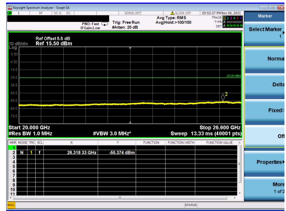
N41(70M)_DFT-s-OFDM_BPSK_Edge_1RB_Left_ Low_CH
