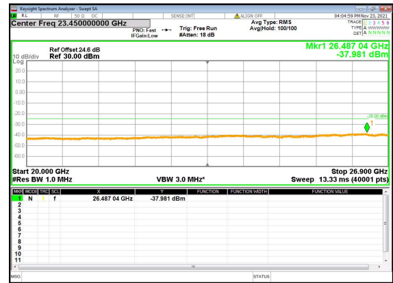
N41(90M)_DFT-s-OFDM_BPSK_Edge_1RB_Left_ Low_CH
