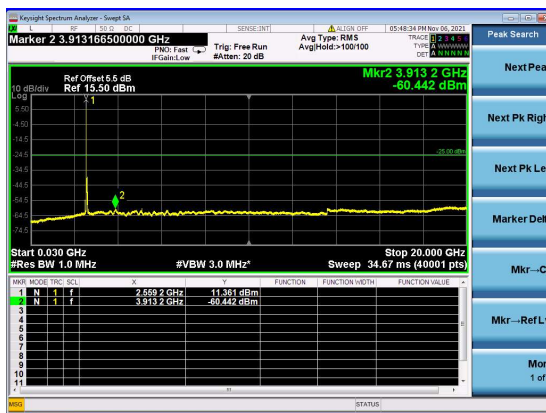
N41(70M)_DFT-s-OFDM_BPSK_Edge_1RB_Left_ Mid_CH
