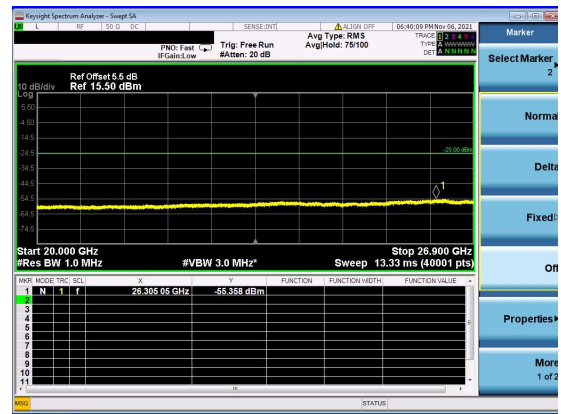
N41(70M)_DFT-s-OFDM_BPSK_Edge_1RB_Left_High_CH
