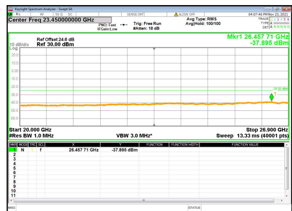
N41(90M)_DFT-s-OFDM_BPSK_Edge_1RB_Left_ Mid_CH
