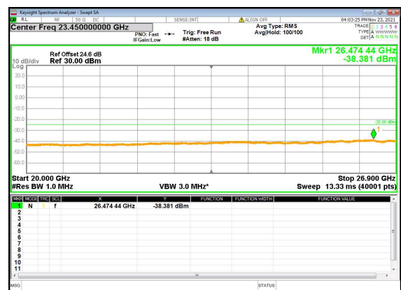
N41(80M)_DFT-s-OFDM_QPSK_Edge_1RB_Left_High_CH
