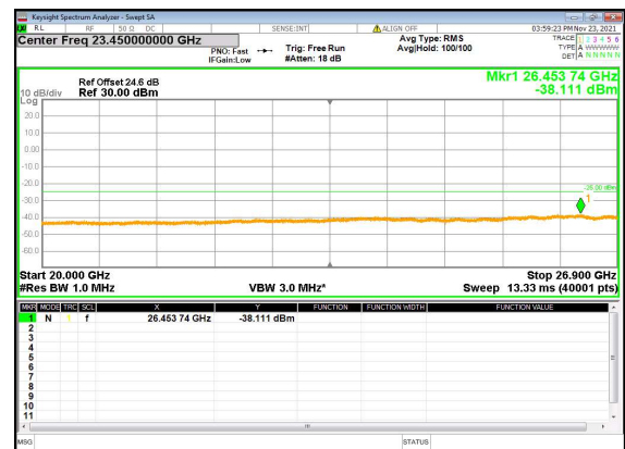
N41(80M)_DFT-s-OFDM_BPSK_Edge_1RB_Left_ Mid_CH
