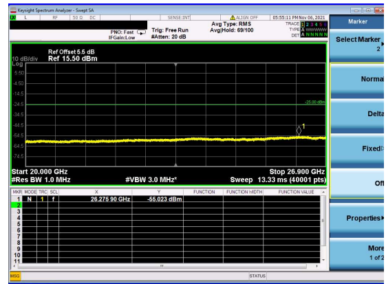
N41(70M)_DFT-s-OFDM_QPSK_Edge_1RB_Left_Mid_CH
