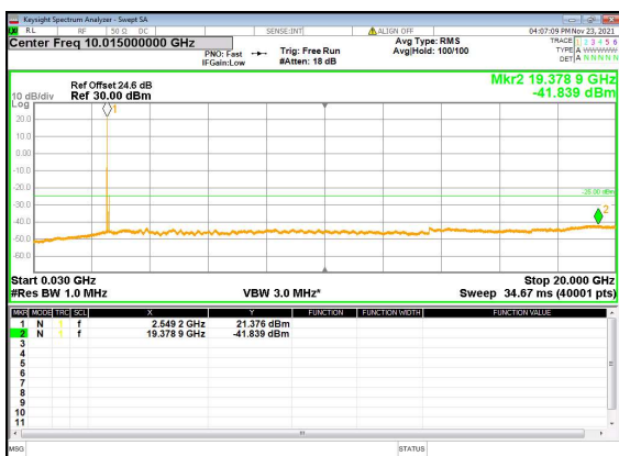
N41(90M)_DFT-s-OFDM_BPSK_Edge_1RB_Left_ Mid_CH
