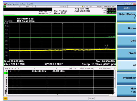
N41(70M)_DFT-s-OFDM_QPSK_Edge_1RB_Left_ Low_CH
