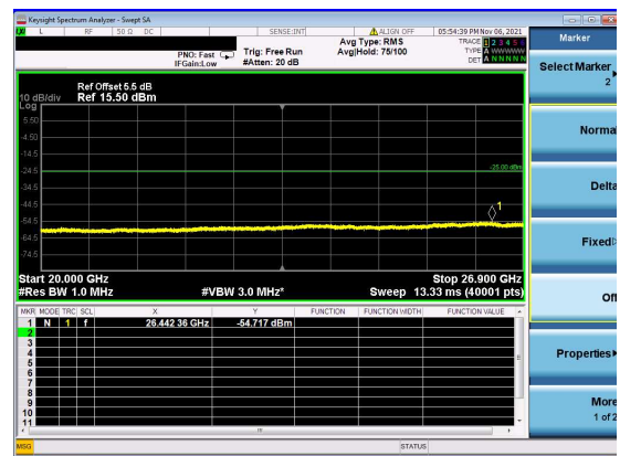
N41(70M)_DFT-s-OFDM_BPSK_Edge_1RB_Left_ Mid_CH
