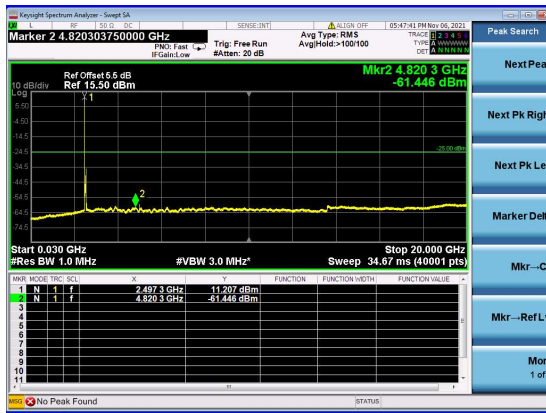
N41(70M)_DFT-s-OFDM_BPSK_Edge_1RB_Left_ Low_CH
