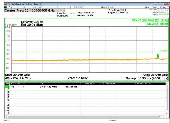
N41(80M)_DFT-s-OFDM_BPSK_Edge_1RB_Left_High_CH
