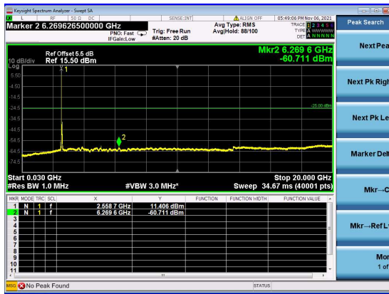
N41(70M)_DFT-s-OFDM_QPSK_Edge_1RB_Left_Mid_CH
