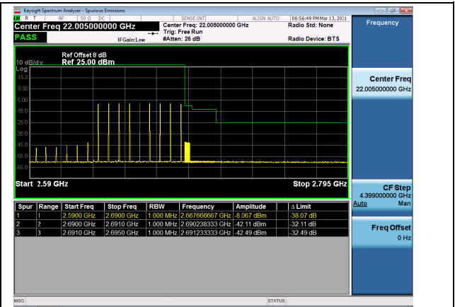
N41(60M)_DFT-s-OFDM_QPSK_Edge_1RB_High_CH
