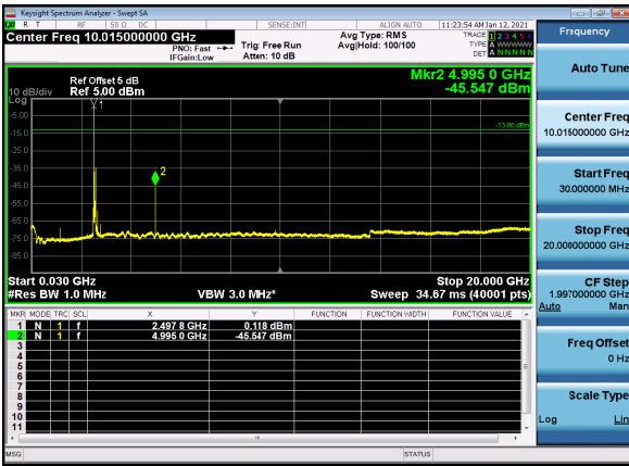
N41(80M)_DFT-s-OFDM_BPSK_Edge_1RB_Low_CH
