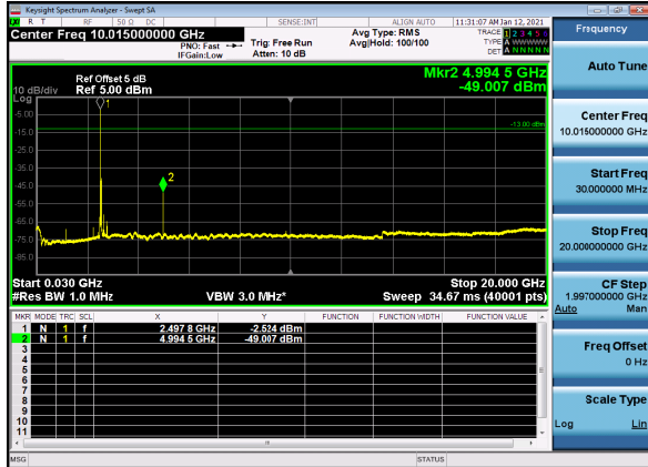
N41(60M)_DFT-s-OFDM_BPSK_Edge_1RB_Low_CH
