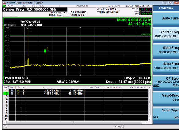
N41(20M)_DFT-s-OFDM_QPSK_Edge_1RB_Low_CH
