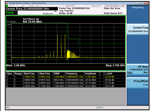
N41(20M)_DFT-s-OFDM_QPSK_Outer_Full_High_CH
