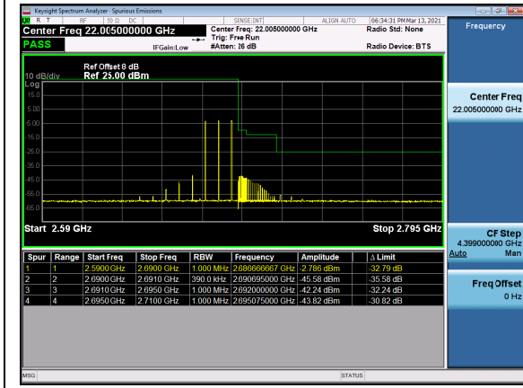
N41(20M)_DFT-s-OFDM_BPSK_Outer_Full_High_CH
