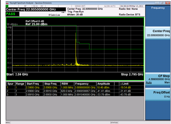
N41(40M)_DFT-s-OFDM_QPSK_Outer_Full_High_CH
