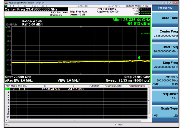
N41(20M)_DFT-s-OFDM_QPSK_Edge_1RB_Low_CH
