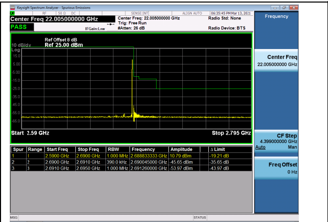
N41(20M)_DFT-s-OFDM_QPSK_Outer_Full_High_CH
