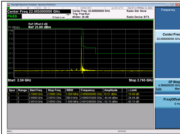
N41(20M)_DFT-s-OFDM_BPSK_Outer_Full_High_CH
