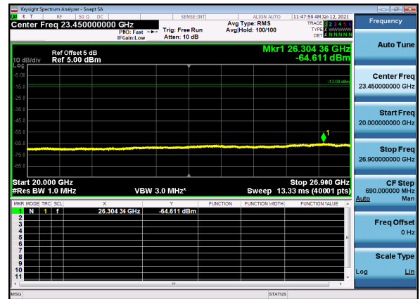
N41(20M)_DFT-s-OFDM_BPSK_Edge_1RB_Mid_CH
