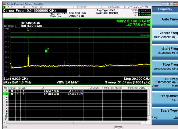
N41(20M)_DFT-s-OFDM_BPSK_Edge_1RB_Mid_CH
