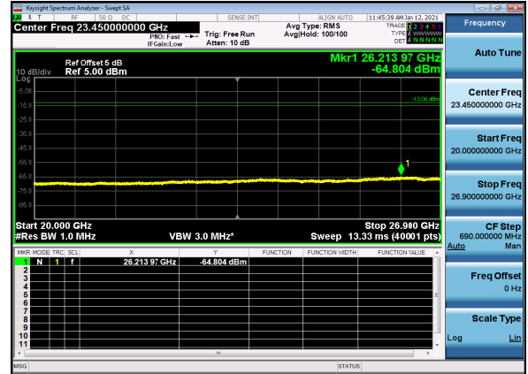
N41(20M)_DFT-s-OFDM_BPSK_Edge_1RB_Low_CH
