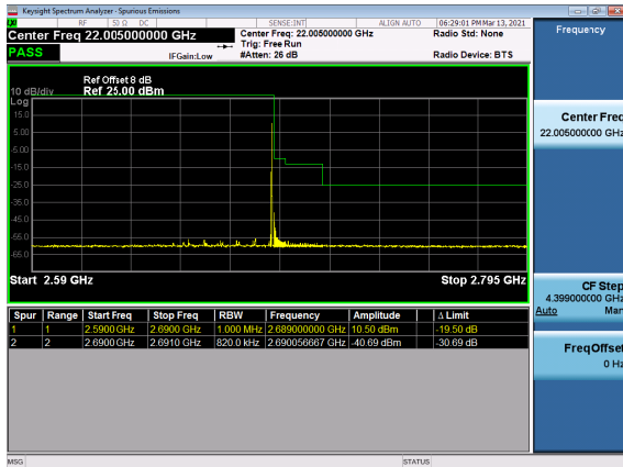
N41(40M)_DFT-s-OFDM_BPSK_Outer_Full_High_CH
