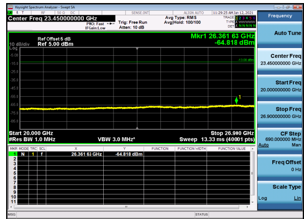
N41(80M)_DFT-s-OFDM_BPSK_Edge_1RB_High_CH
