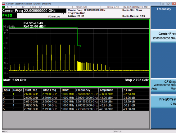
N41(40M)_DFT-s-OFDM_BPSK_Edge_1RB_Low_CH
