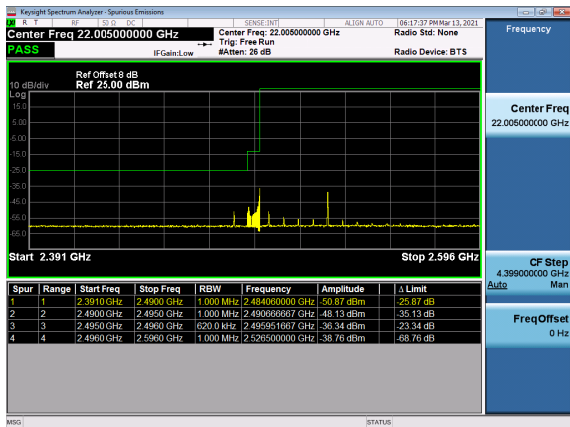
N41(60M)_DFT-s-OFDM_BPSK_Outer_Full_Low_CH
