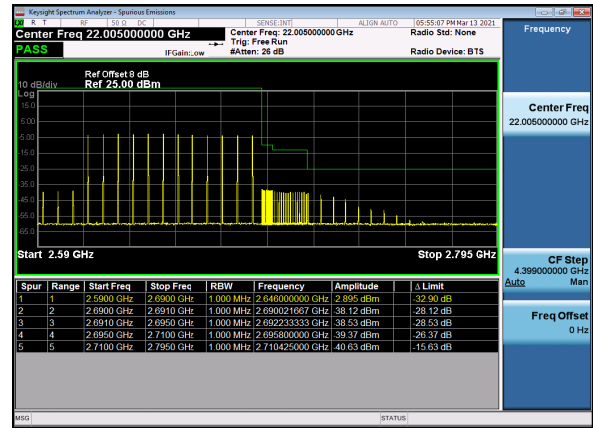
N41(60M)_DFT-s-OFDM_QPSK_Edge_1RB_Low_CH
