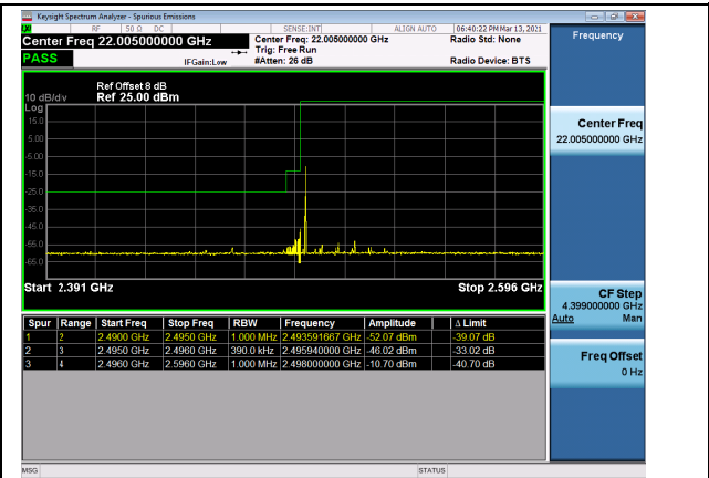
N41(40M)_DFT-s-OFDM_QPSK_Outer_Full_Low_CH
