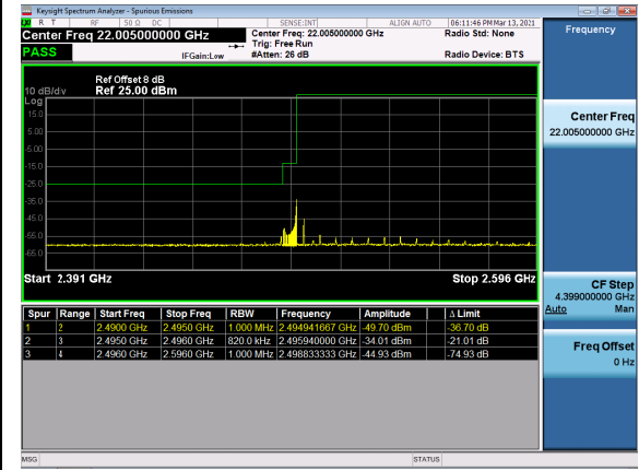
N41(80M)_DFT-s-OFDM_QPSK_Outer_Full_Low_CH
