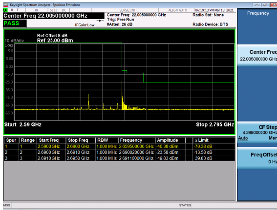
N41(60M)_DFT-s-OFDM_BPSK_Outer_Full_High_CH
