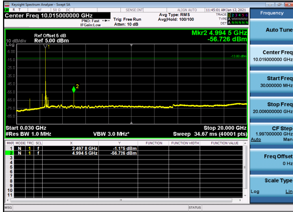
N41(20M)_DFT-s-OFDM_BPSK_Edge_1RB_Low_CH
