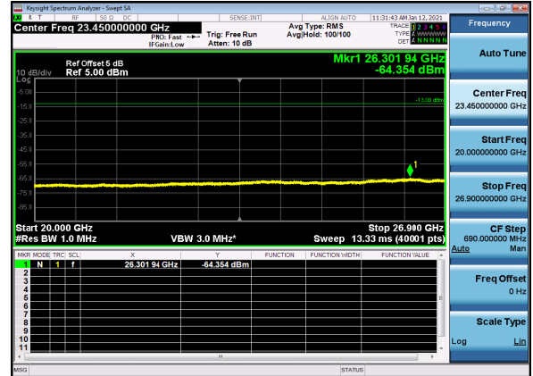
N41(60M)_DFT-s-OFDM_BPSK_Edge_1RB_Low_CH
