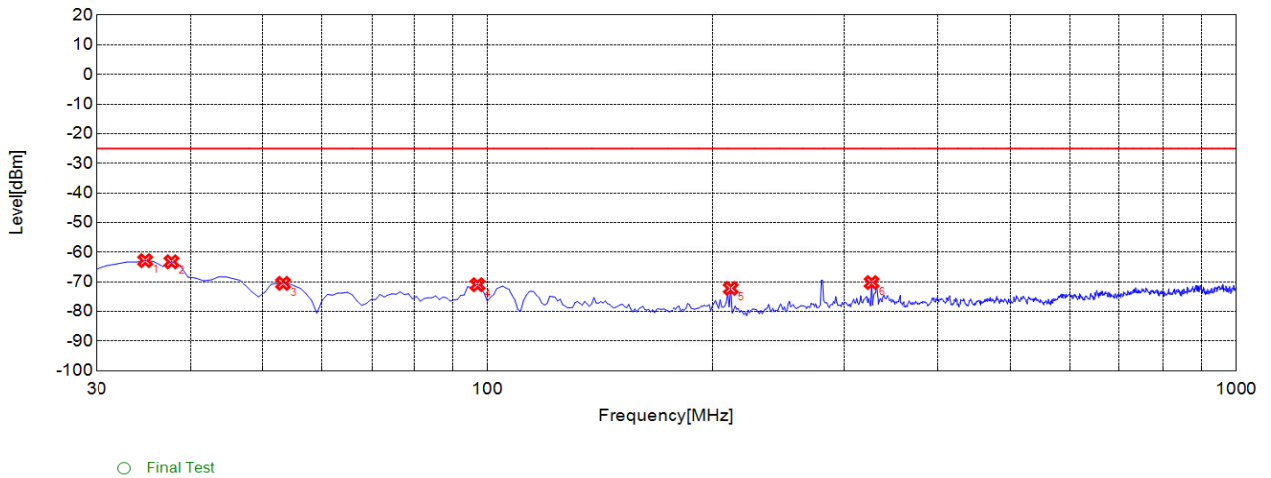
n41 534000 40Mhz CP-OFDM 16 QAM 1RB_Right 30M-1G V
