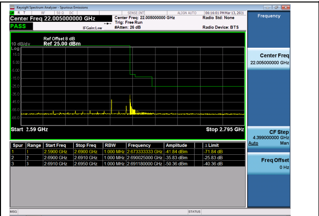
N41(80M)_DFT-s-OFDM_QPSK_Outer_Full_High_CH
