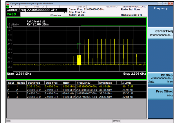
N41(80M)_DFT-s-OFDM_QPSK_Edge_1RB_High_CH
