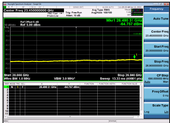
N41(80M)_DFT-s-OFDM_QPSK_Edge_1RB_Low_CH
