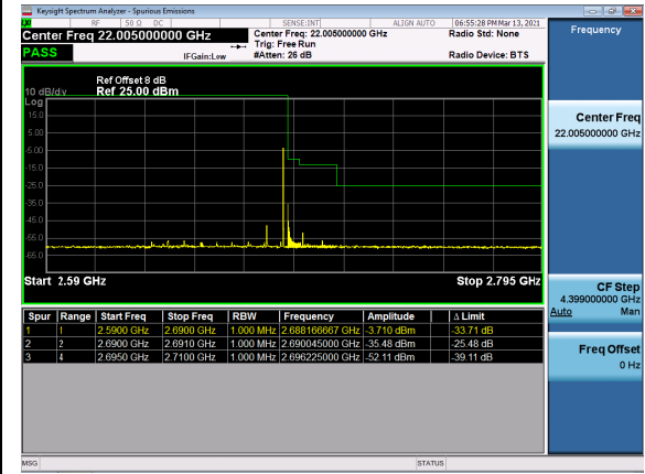
N41(60M)_DFT-s-OFDM_QPSK_Outer_Full_High_CH
