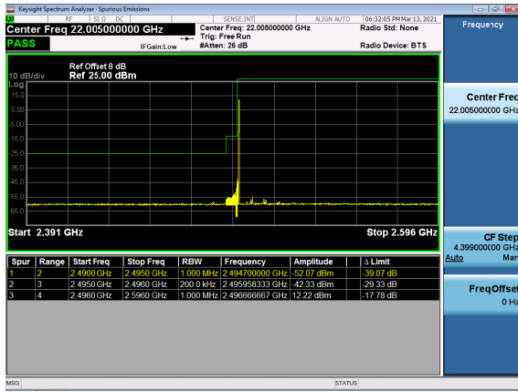
N41(20M)_DFT-s-OFDM_BPSK_Outer_Full_Low_CH
