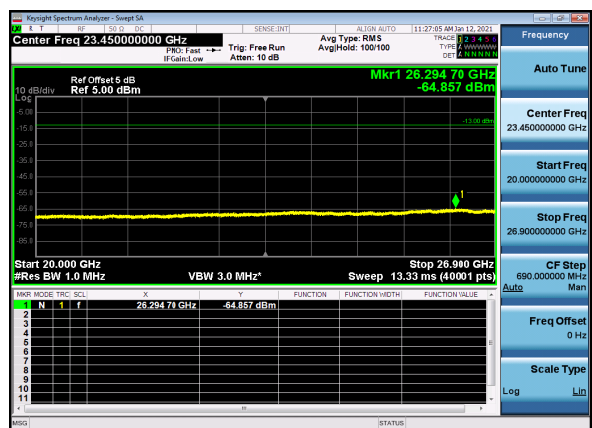
N41(80M)_DFT-s-OFDM_BPSK_Edge_1RB_Mid_CH
