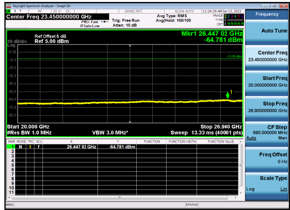
N41(80M)_DFT-s-OFDM_BPSK_Edge_1RB_Low_CH
