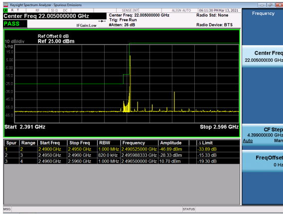
N41(80M)_DFT-s-OFDM_BPSK_Outer_Full_Low_CH
