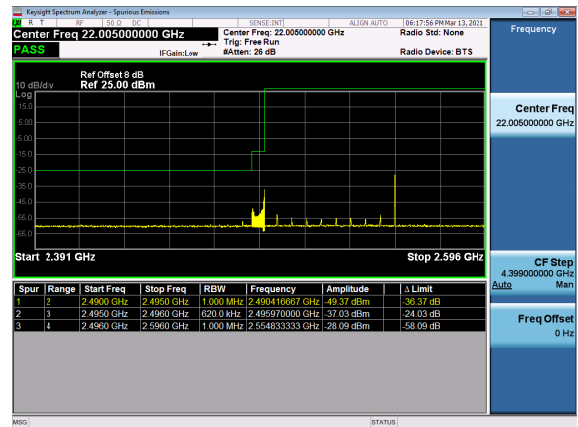
N41(60M)_DFT-s-OFDM_QPSK_Outer_Full_Low_CH
