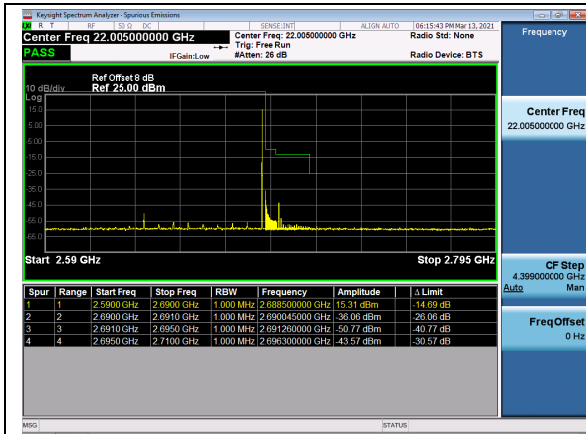
N41(80M)_DFT-s-OFDM_BPSK_Outer_Full_High_CH
