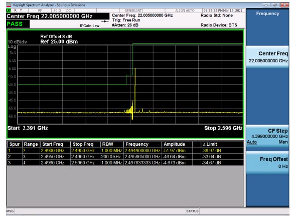
N41(20M)_DFT-s-OFDM_QPSK_Outer_Full_Low_CH
