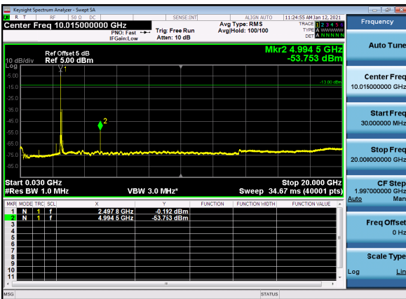
N41(80M)_DFT-s-OFDM_QPSK_Edge_1RB_Low_CH
