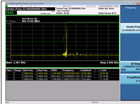
N41(40M)_DFT-s-OFDM_BPSK_Outer_Full_Low_CH
