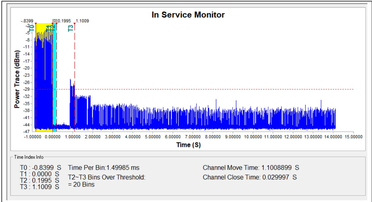
(5290MHz, 802.11ax(HEW80))
