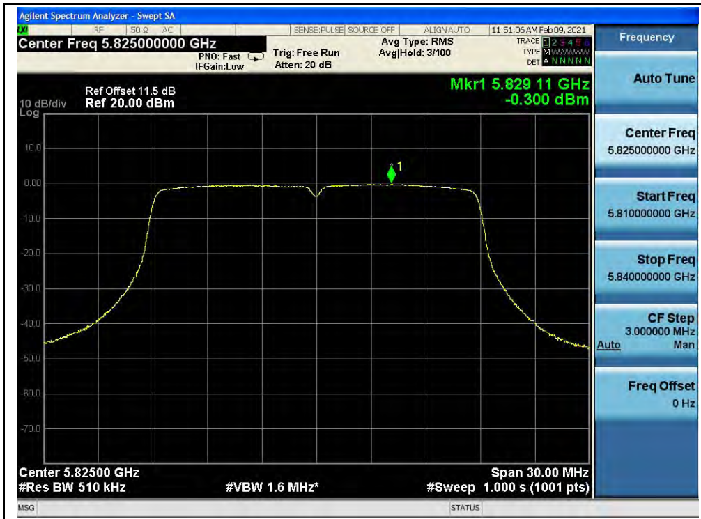
(Channel 165, 5825MHz, 802.11n (HT20), ANTO)
