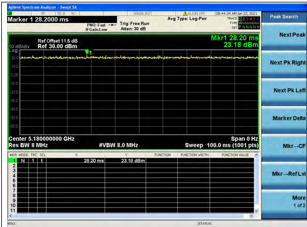
(CH36_5180MHz_802.11 ax(HEW20))
