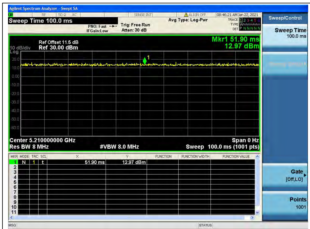
(CH42_5210MHz_802.11 ax(HEW80))
