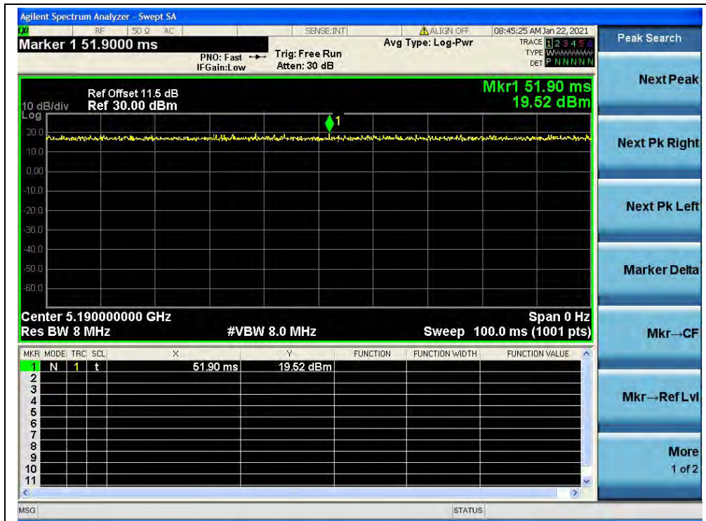
(CH38_5190MHz_802.11 ax(HEW40))
