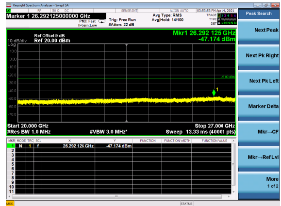
B2_N41(50M)_DFT-s-OFDM_QPSK_Edg e_1RB_Left_High_CH
