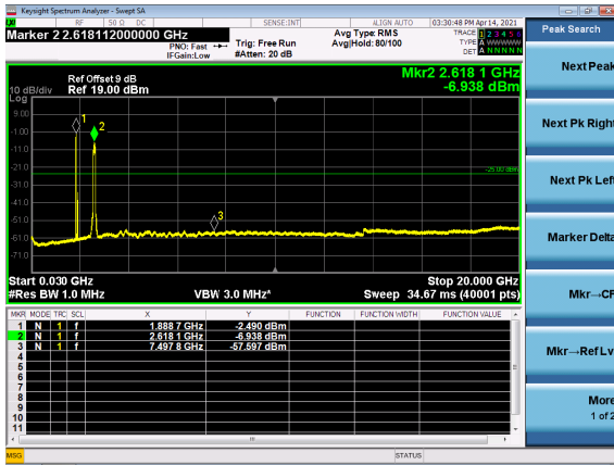
B2_N41(90M)_DFT-s-OFDM_BPSK_Edge_1 RB_Left_High_CH
