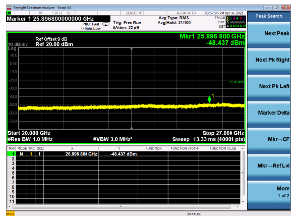
B2_N41(60M)_DFT-s-OFDM_QPSK_Edg e_1RB_Left_Low_CH
