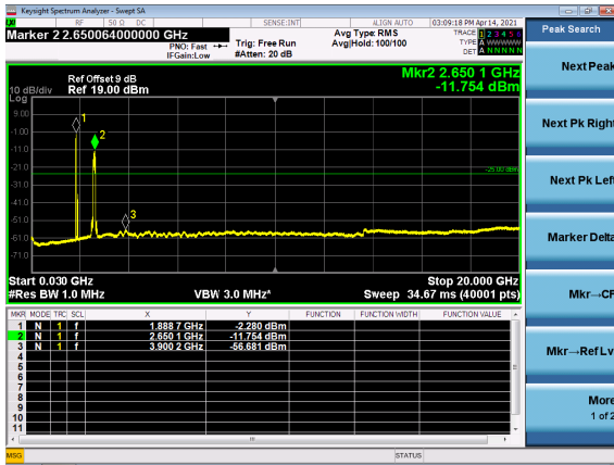
B2_N41(100M)_DFT-s-OFDM_BPSK_Edge_1RB_Left_High_CH
