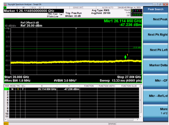
B2_N41(100M)_DFT-s-OFDM_BPSK_Edge_1RB_Left_Mid_CH
