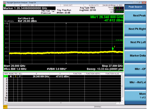
B2_N41(100M)_DFT-s-OFDM_BPSK_Edge_1RB_Left_High_CH
