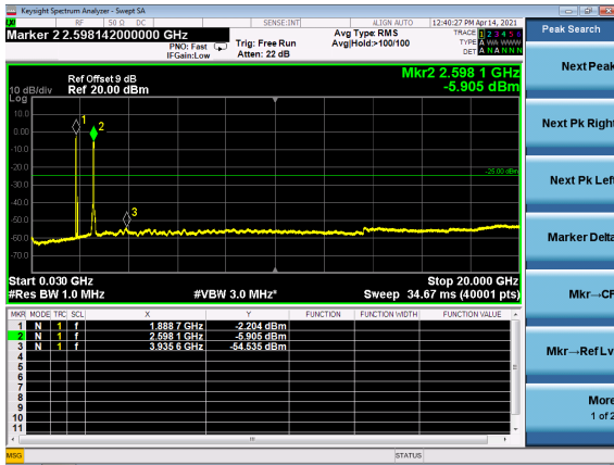
B2_N41(60M)_DFT-s-OFDM_QPSK_Edge_1 RB_Left_Mid_CH
