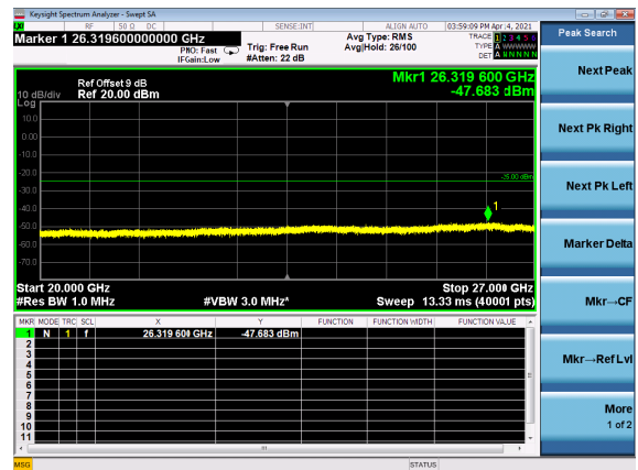
B2_N41(90M)_DFT-s-OFDM_QPSK_Edg e_1RB_Left_High_CH
