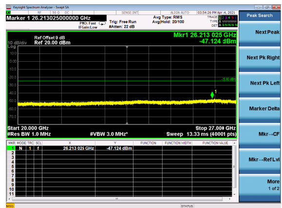
B2_N41(50M)_DFT-s-OFDM_BPSK_Edg e_1RB_Left_Mid_CH
