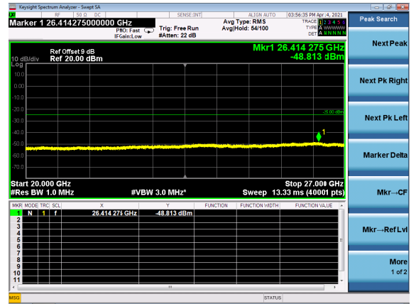
B2_N41(60M)_DFT-s-OFDM_QPSK_Edg e_1RB_Left_Mid_CH
