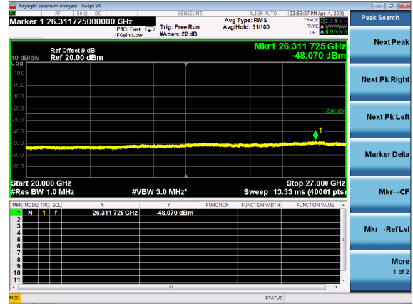
B2_N41(50M)_DFT-s-OFDM_BPSK_Edg e_1RB_Left_High_CH
