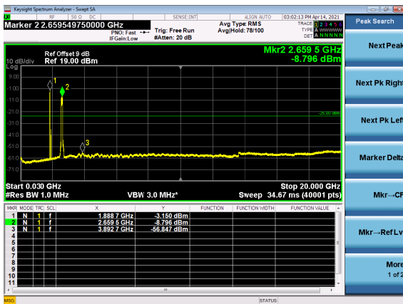
B2_N41(90M)_DFT-s-OFDM_QPSK_Edge_ 1RB_Left_High_CH
