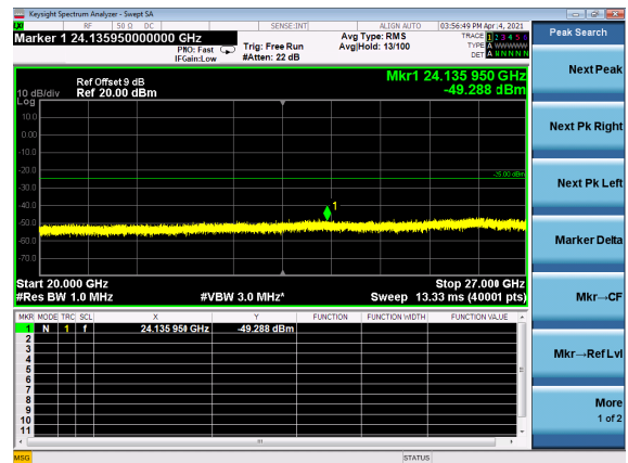
B2_N41(60M)_DFT-s-OFDM_BPSK_Edg e_1RB_Left_Low_CH
