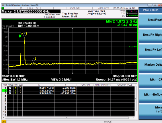
B2_N41(90M)_DFT-s-OFDM_BPSK_Edge_ 1RB_Left_Mid_CH
