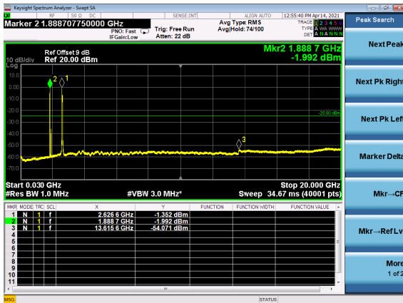
B2_N41(50M)_DFT-s-OFDM_QPSK_Edge_ 1RB_Left_High_CH
