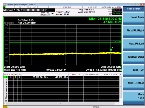
B2_N41(90M)_DFT-s-OFDM_BPSK_Edg e_1RB_Left_Mid_CH
