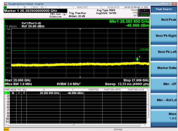
B2_N41(100M)_DFT-s-OFDM_QPSK_Edge_1RB_Left_High_CH
