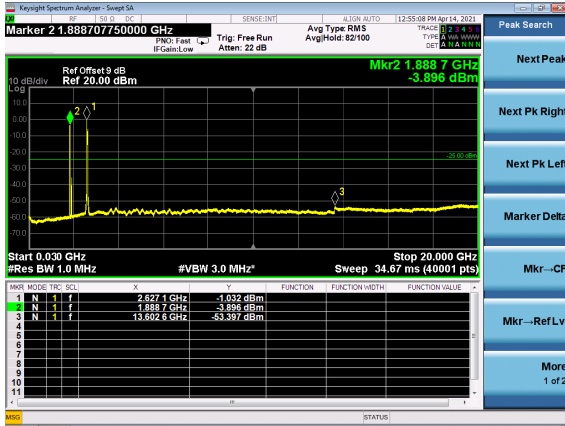
B2_N41(50M)_DFT-s-OFDM_BPSK_Edge_1 RB_Left_High_CH
