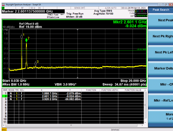
B2_N41(100M)_DFT-s-OFDM_BPSK_Edge_1RB_Left_Mid_CH
