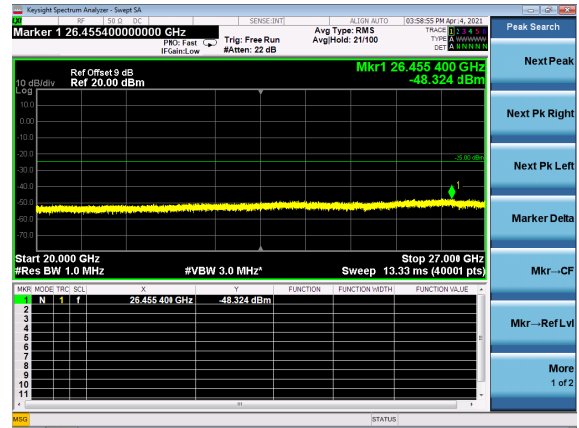
B2_N41(90M)_DFT-s-OFDM_BPSK_Edg e_1RB_Left_High_CH
