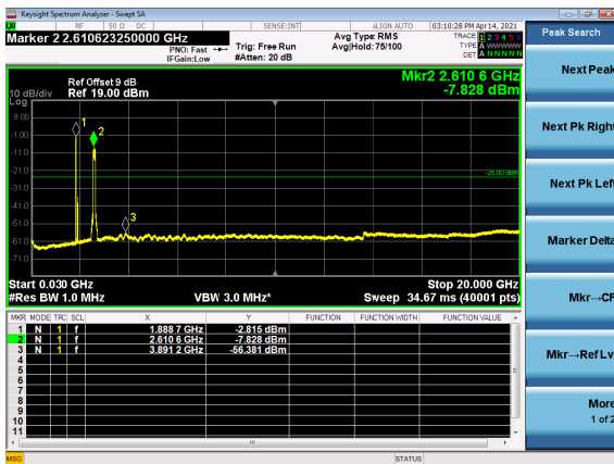
B2_N41(100M)_DFT-s-OFDM_QPSK_Edge_1RB_Left_High_CH
