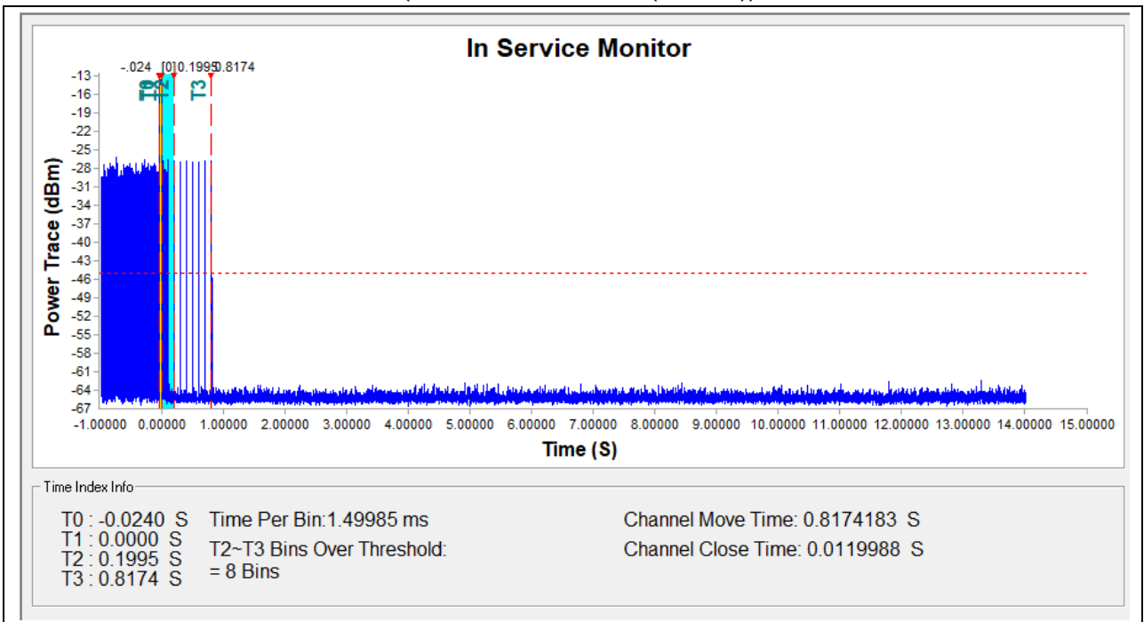
(5280MHz, 802.11 ac (VHT20))
