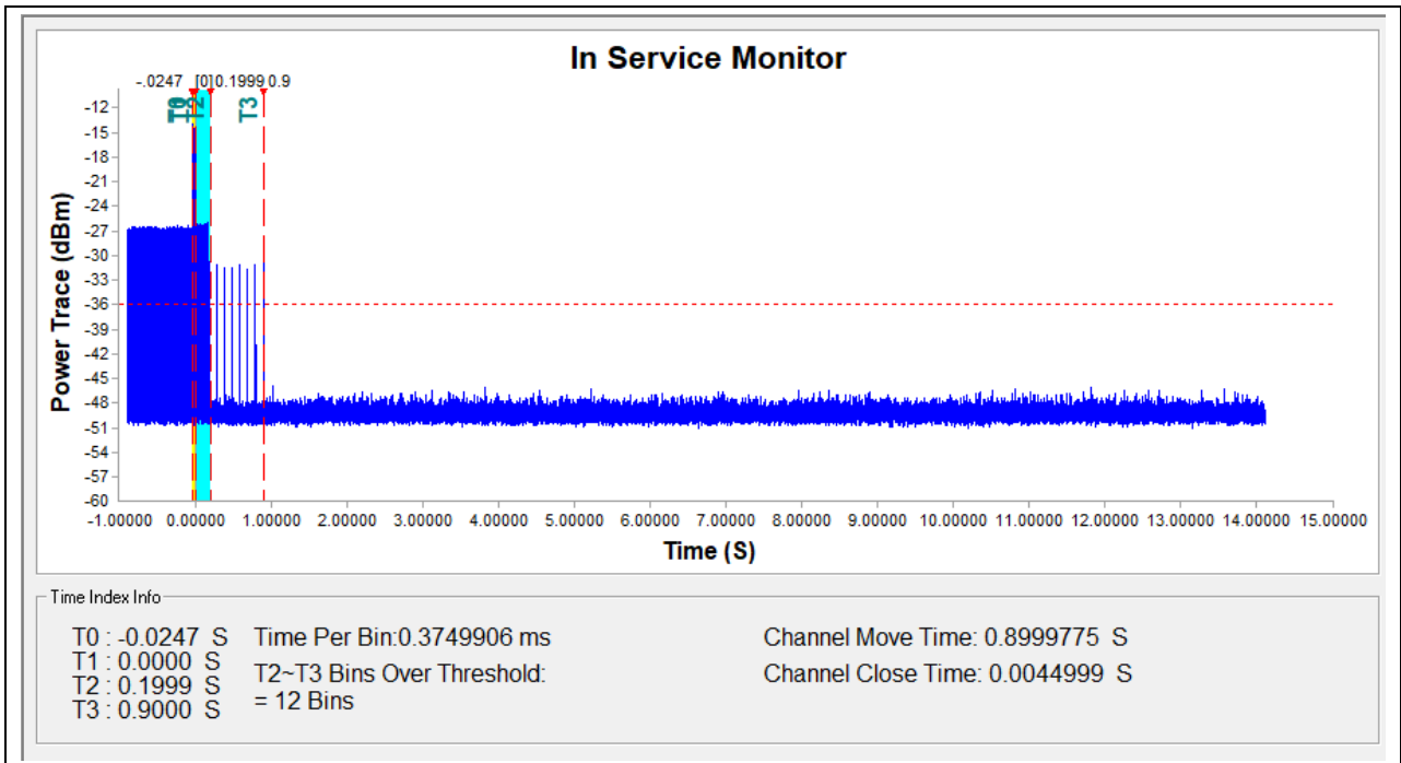
(5640MHz, 802.11ac (VHT20))
