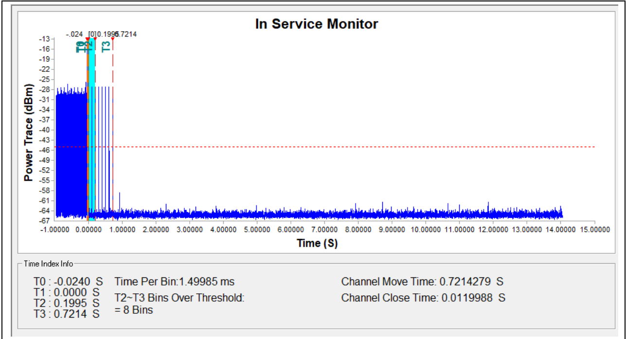
(5260MHz, 802.11ac (VHT20))
