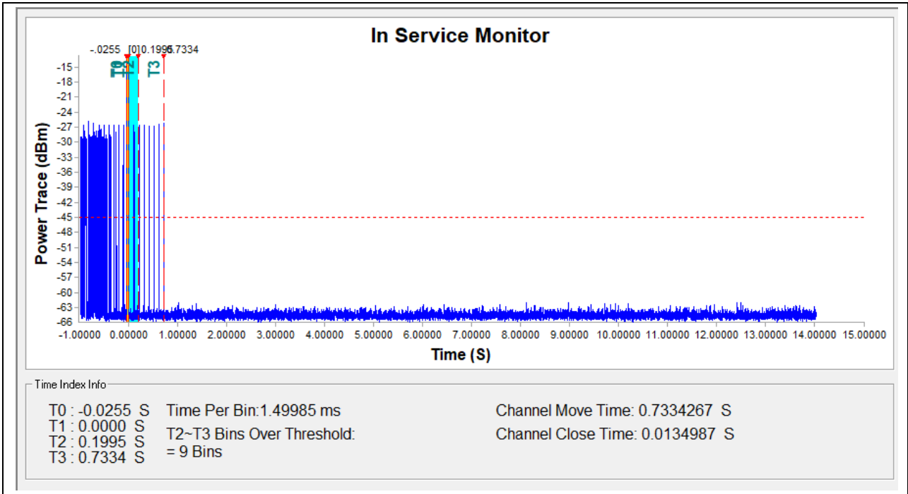
(5580MHz, 802.11 ac (VHT20))
