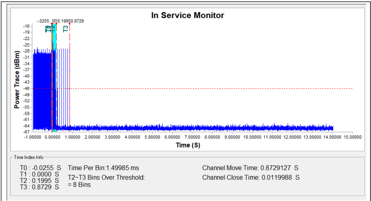
(5320MHz, 802.11ac (VHT20))
