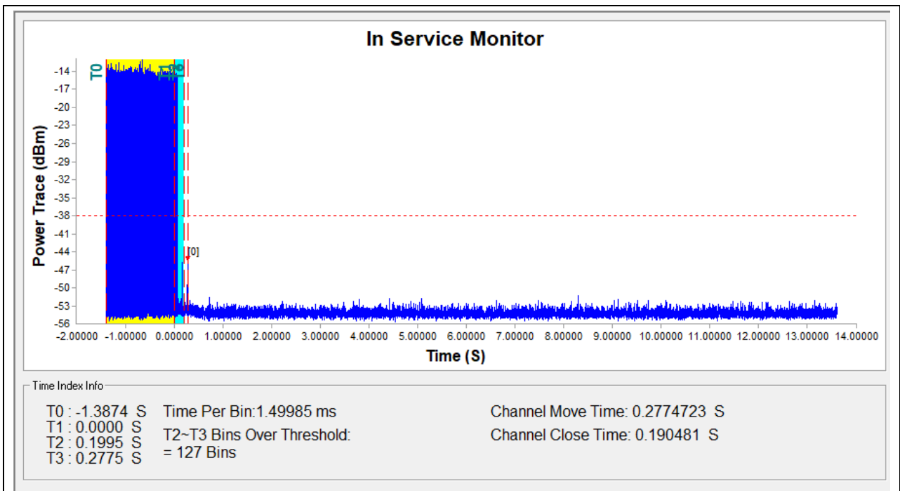
(5530MHz, 802.11ax (HEW80))
