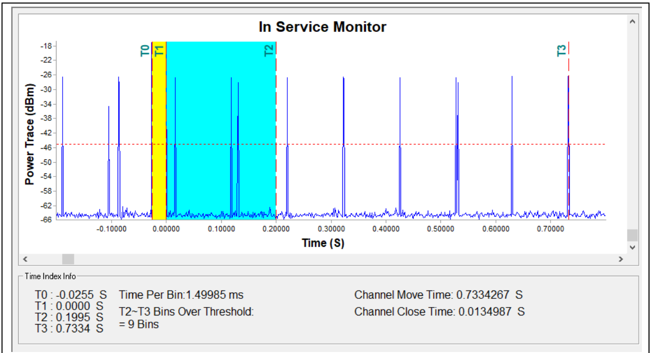
(5580MHz, 802.11 ac (VHT20))
