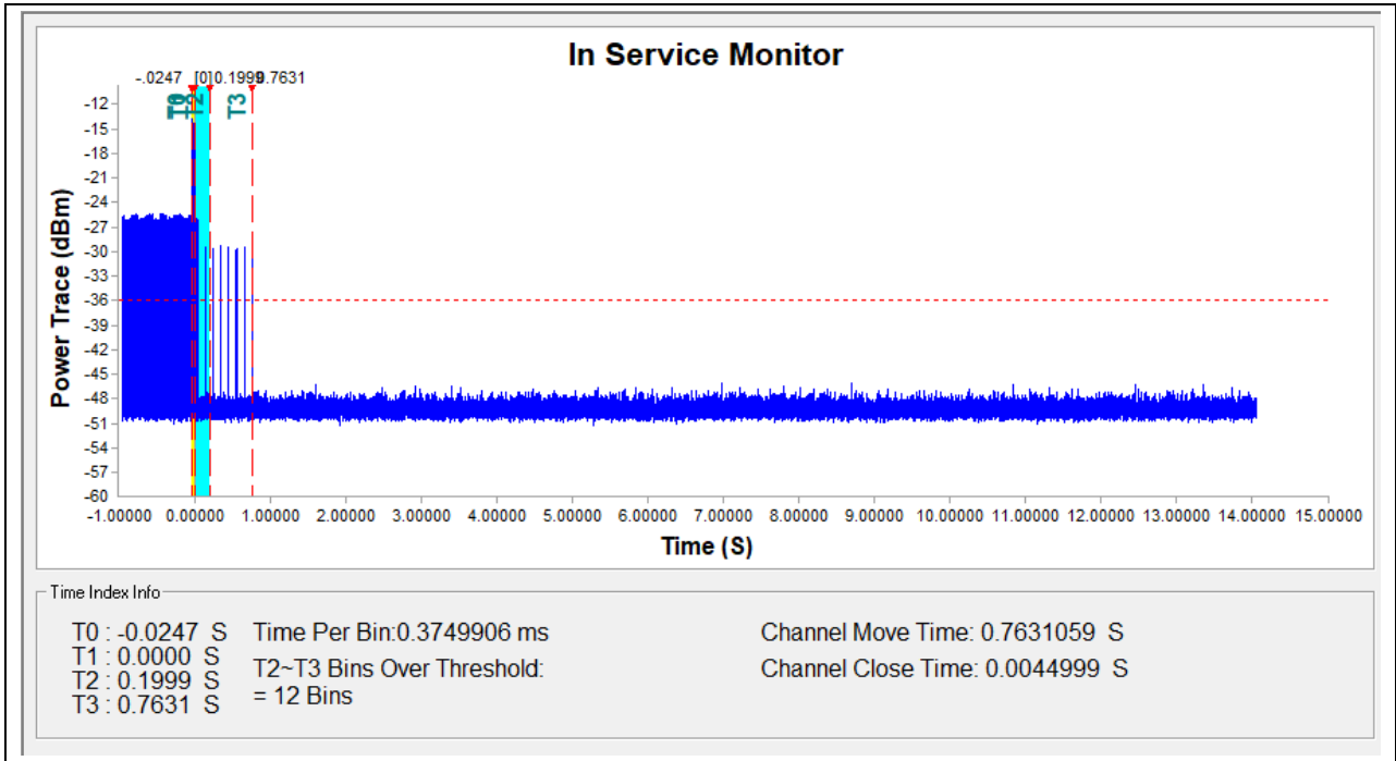
(5620MHz, 802.11ac (VHT20))
