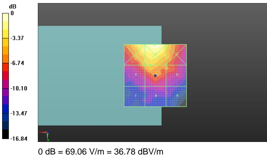
Fig A.1 HAC RF E-Field CDMA BC0
