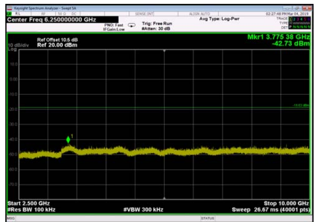
,Plot 4,2500MHz~10000MHz-802.11n(HT40),2452MHz,Ant1
