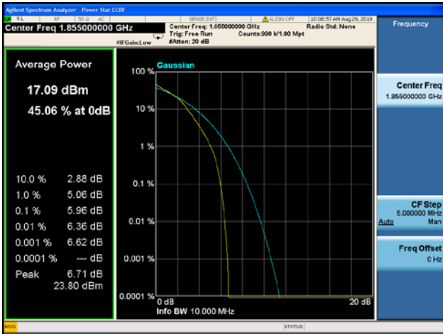
10MHz/16QAM / MCH
