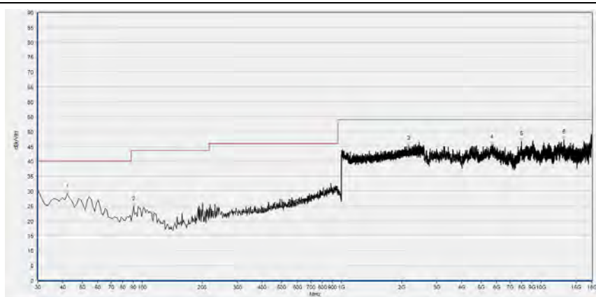
(30MHz to 25GHz, Antenna Horizontal, π/4-DQPSK, channel 39)
