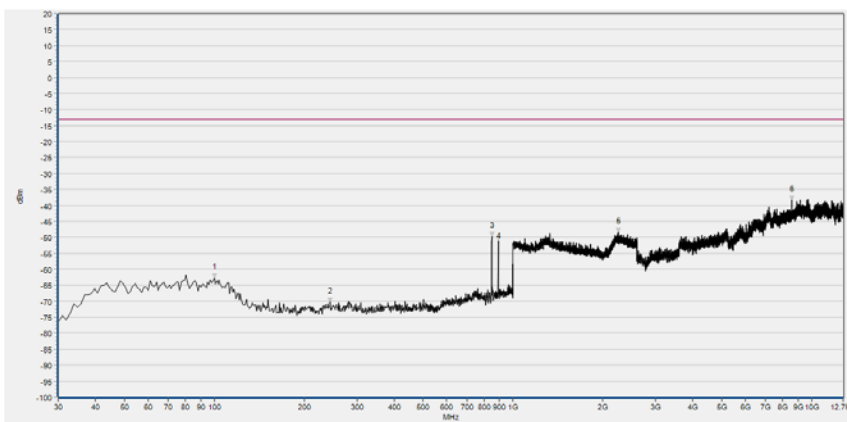
(Plot D4, EVDO B BC0, Channel =384, Vertical)
