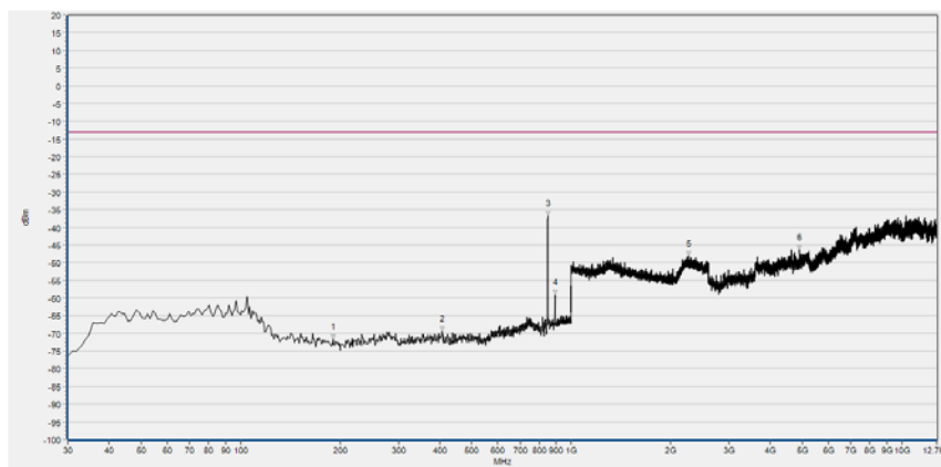
(Plot A4, CDMA BC0, Channel = 384, Vertical)
