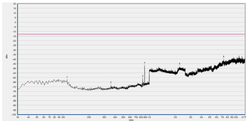
(Plot H3, EVDO B BC0, Channel =384, Horizontal)
