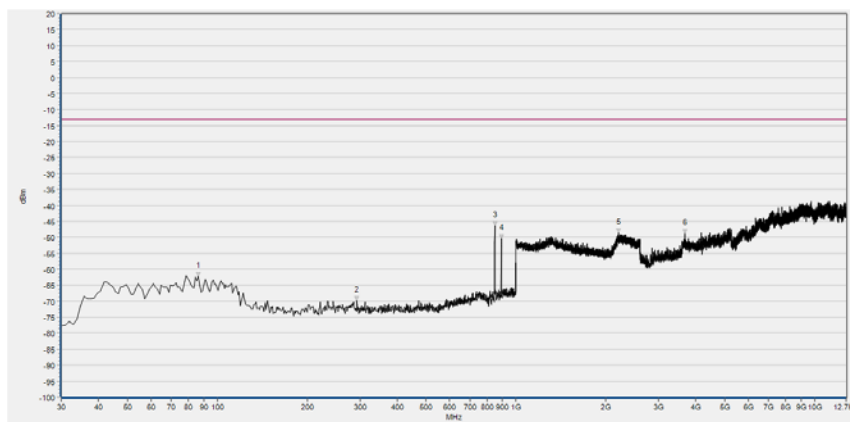
(Plot B4, EVDO 0 BC0, Channel = 384, Vertical)
