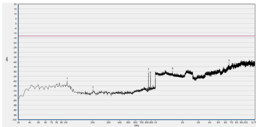
(Plot B2, EVDO 0 BC0, Channel = 1013, Vertical)
