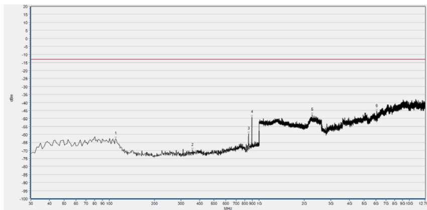
(Plot F5, EVDO 0 BC0, Channel = 777, Horizontal)
