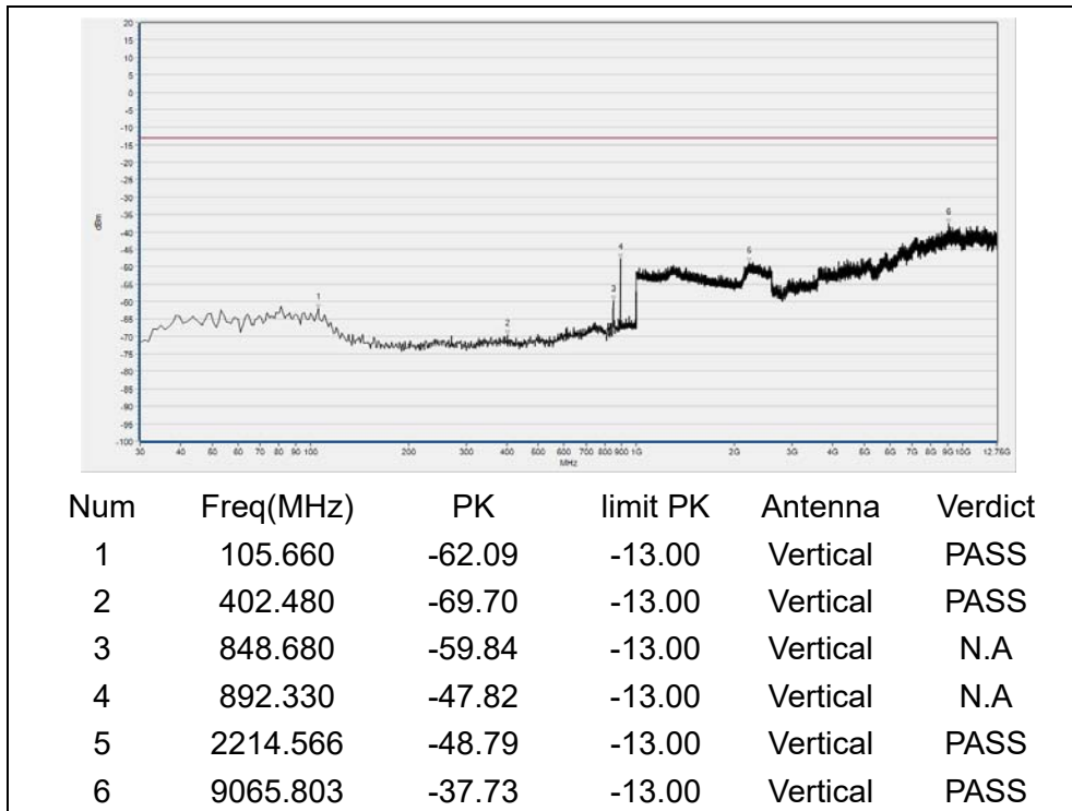
(Plot D6, EVDO B BC0, Channel = 777, Vertical)
