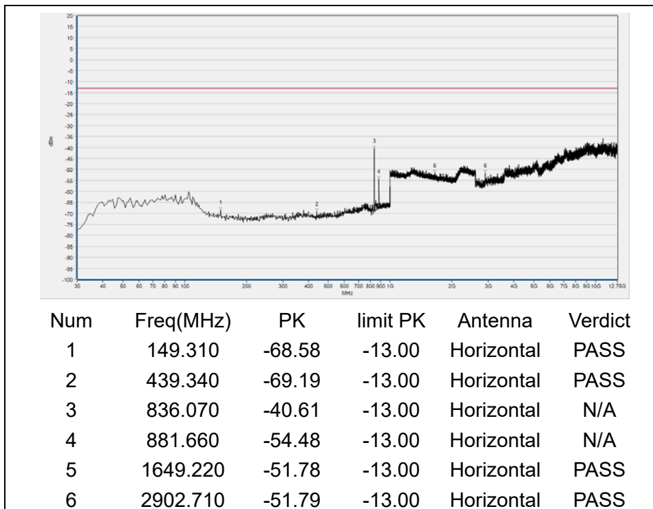
(Plot A3, CDMA BC0, Channel = 384, Horizontal)
