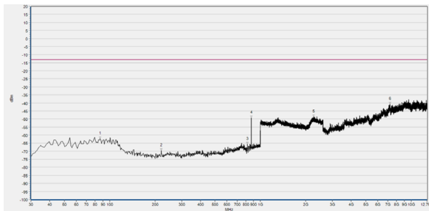
(Plot H1, EVDO B BC0, Channel = 1013, Horizontal)
