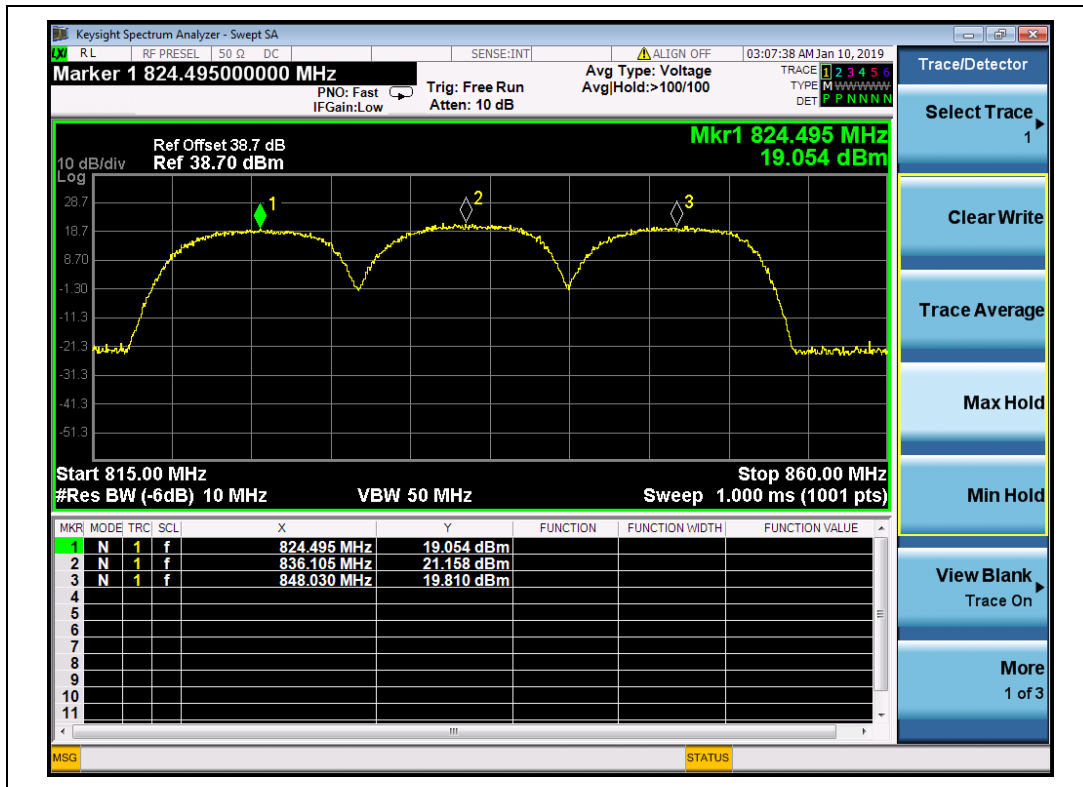
(Plot H, EVDO B BC0, Channel =1013, 384, 777)
