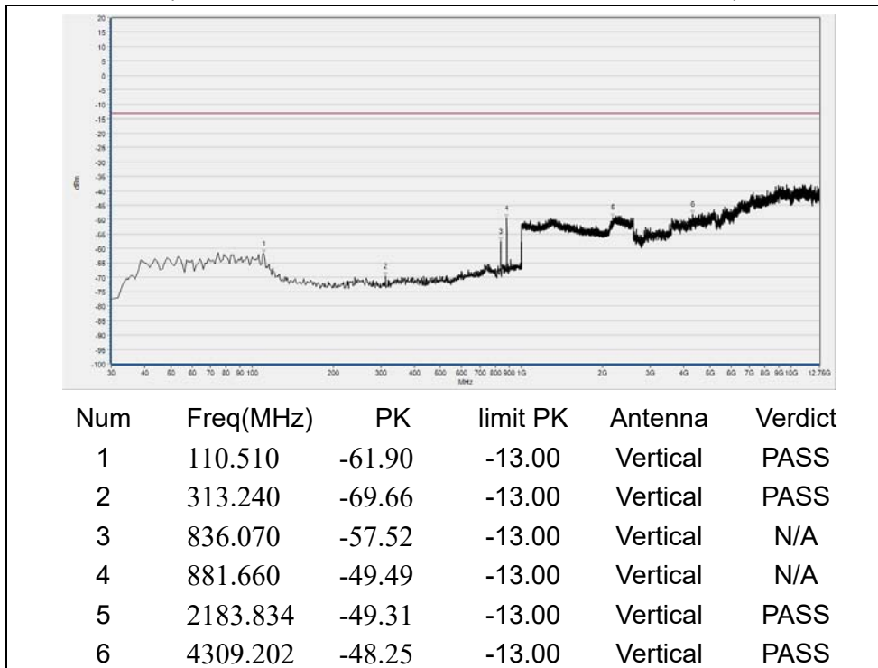
(Plot E4, CDMA BC0, Channel = 384, Vertical)
