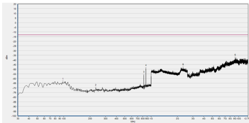
(Plot A6, CDMA BC0, Channel = 777, Vertical)
