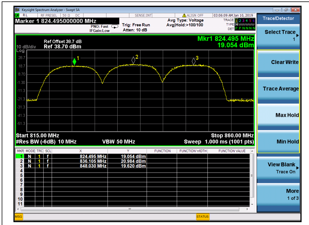
(Plot D, EVDO B BC0, Channel =1013, 384, 777)
