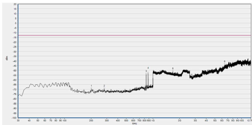
(Plot C2, EVDO A BC0, Channel = 1013, Vertical)
