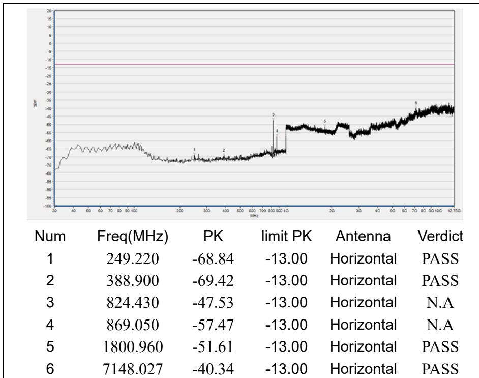
(Plot E1, CDMA BC0, Channel = 1013, Horizontal)
