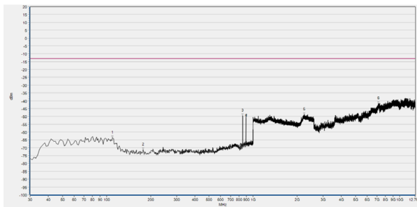
(Plot C4, EVDO A BC0, Channel = 384, Vertical)
