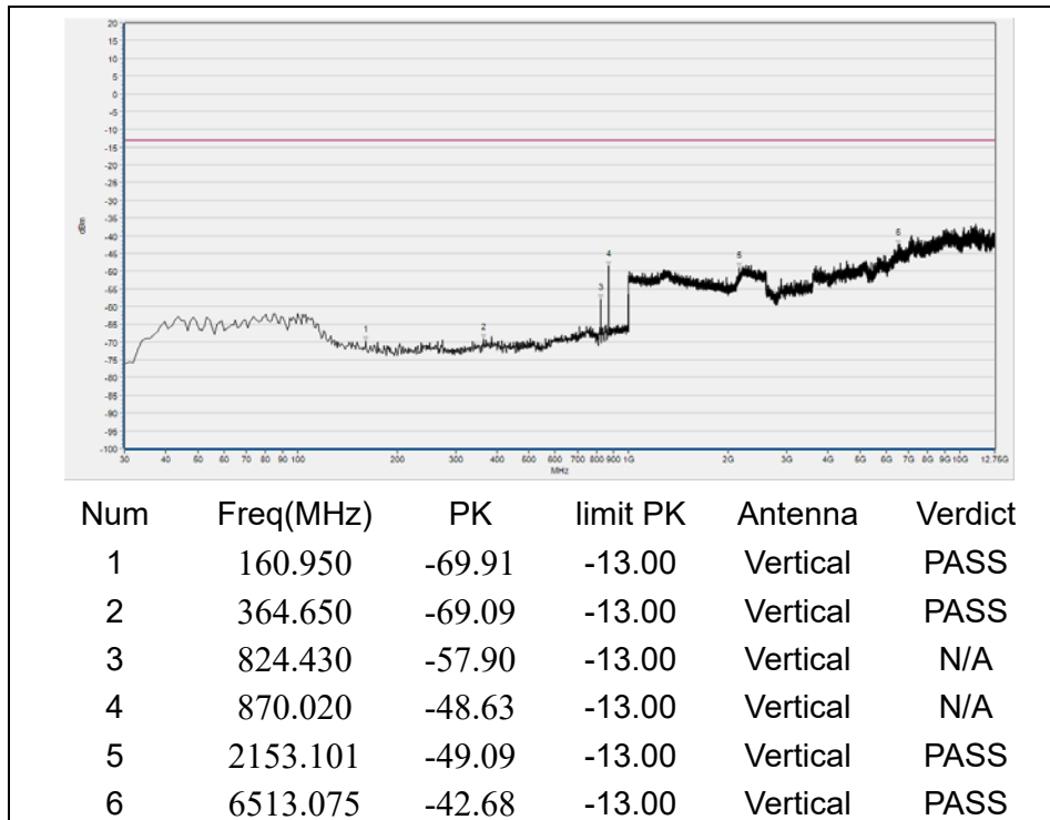
(Plot E2, CDMA BC0, Channel = 1013, Vertical)
