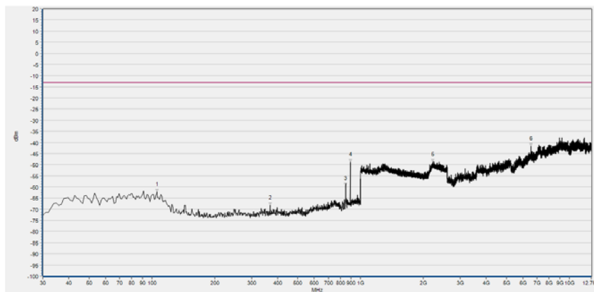
(Plot H5, EVDO B BC0, Channel = 777, Horizontal)
