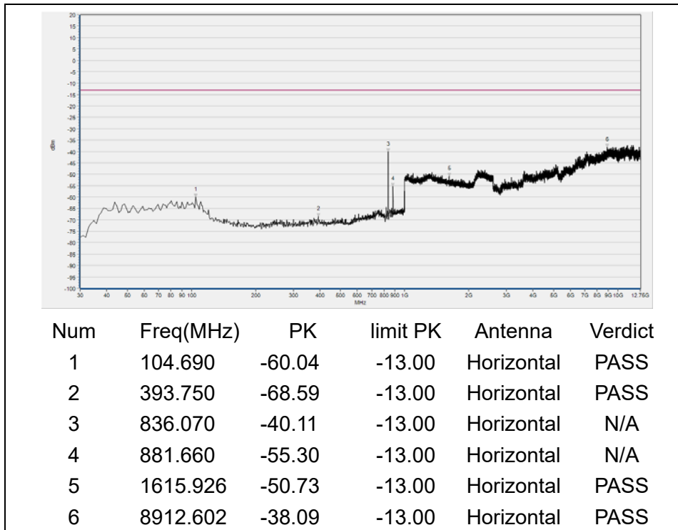
(Plot E3, CDMA BC0, Channel = 384, Horizontal)
