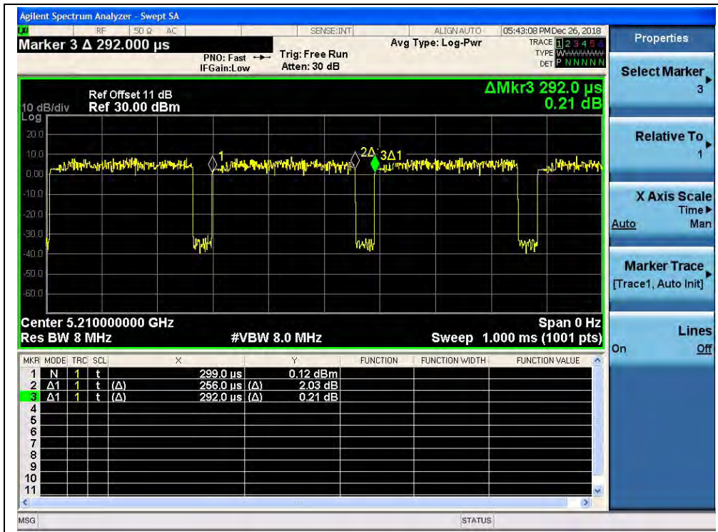
(CH42_5210MHz_802.11 ac(VHT80), ANT1)
