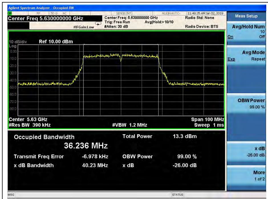
(Channel 126, 5630MHz, 802.11 ac (VHT40), ANT0)
