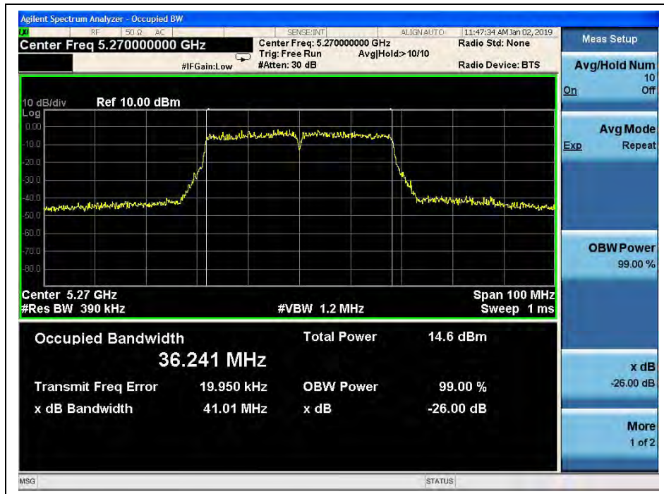
(Channel 54, 5270MHz, 802.11 ac (VHT40), ANT0)
