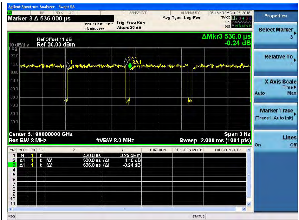
(CH38_5190MHz_802.11 ac(VHT40), ANT0)
