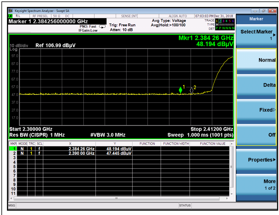
(Channel = 1 PEAK, 802.11b)
