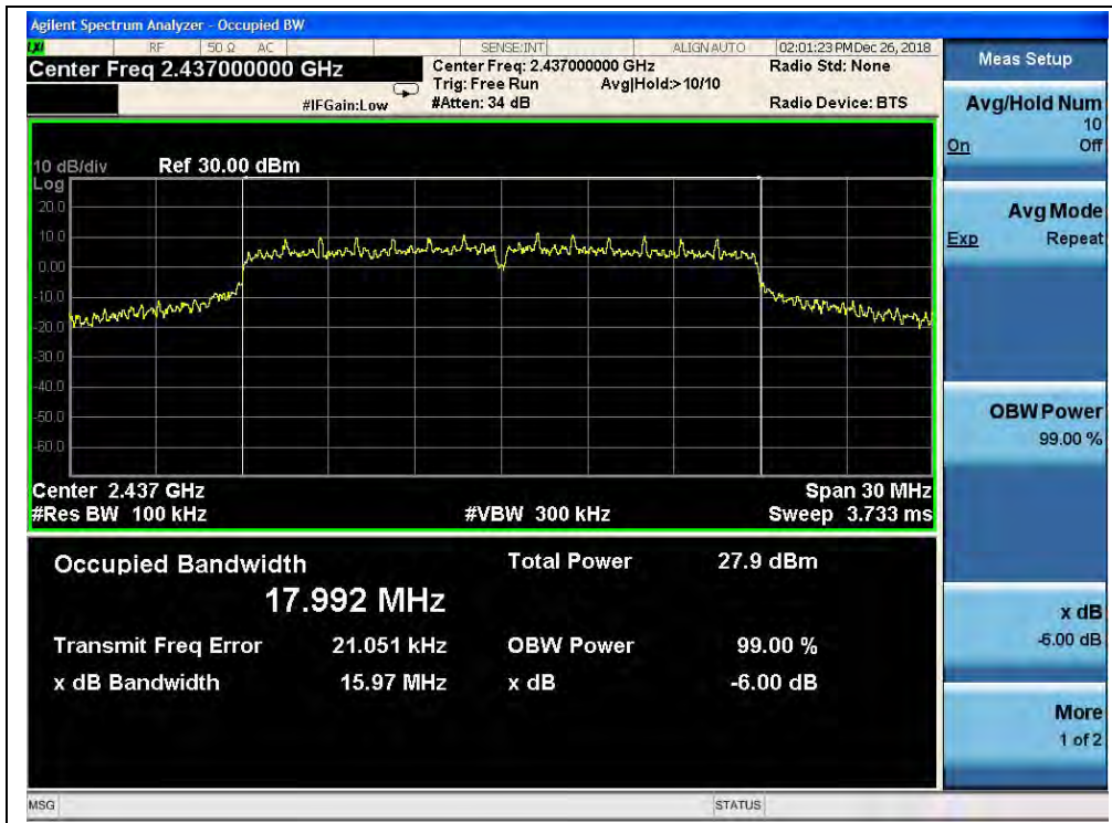
(ANT 1, Channel 6, 2437MHz, 802.11n(HT20))
