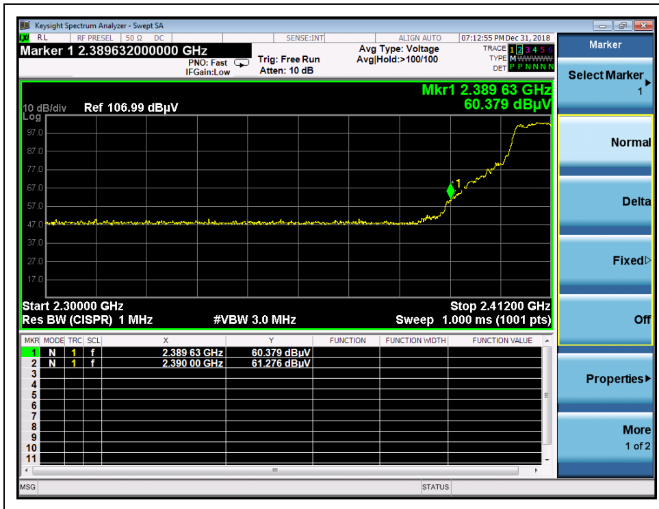
(Channel = 1 PEAK, 802.11g)
