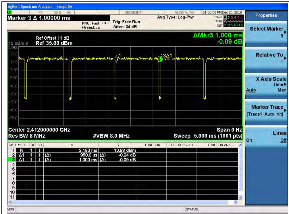
(Channel 1, 2412MHz, 802.11 n(HT40), ANT1)
