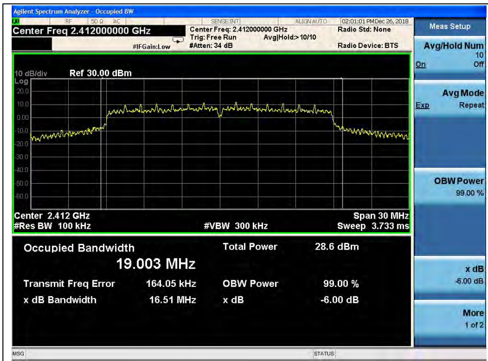
(ANT 1, Channel 1, 2412MHz, 802.11n(HT20))
