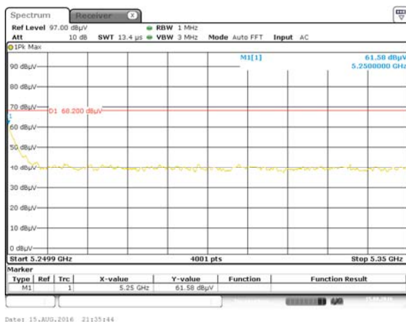
Band I 11n(HT40) CH46, PEAK
