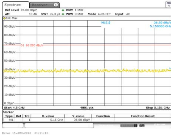
Band I 11a(HT20) CH36, PEAK
