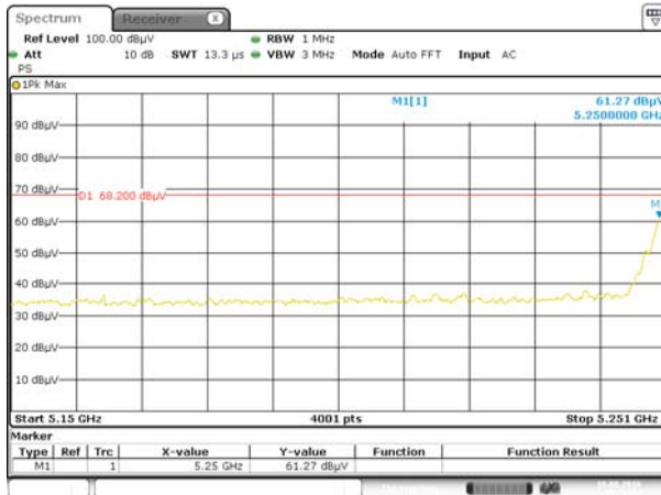
Band II 11a(HT20) CH52, PEAK
