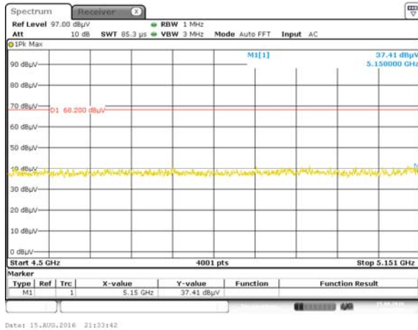
Band I 11n(HT40) CH38, PEAK
