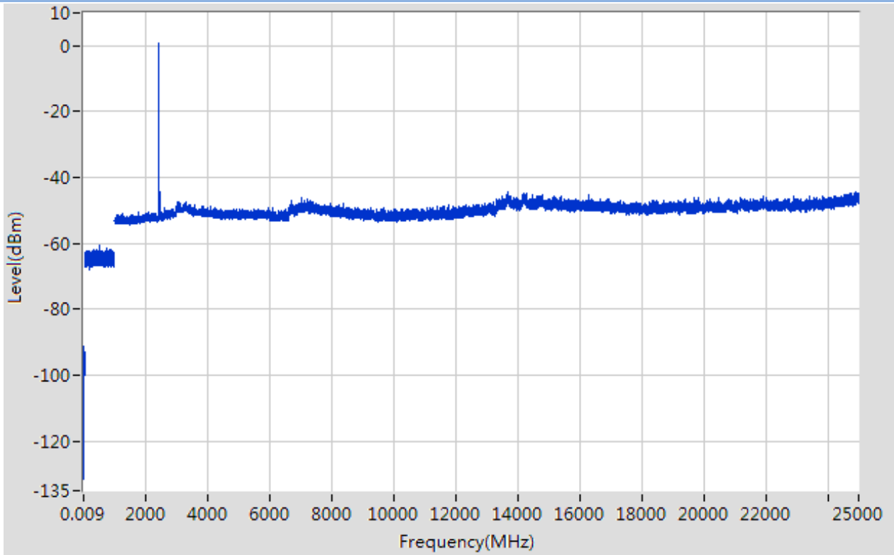
MIDDLE CHANNEL, SPURIOUS 9 kHz ~ 25 GHz
