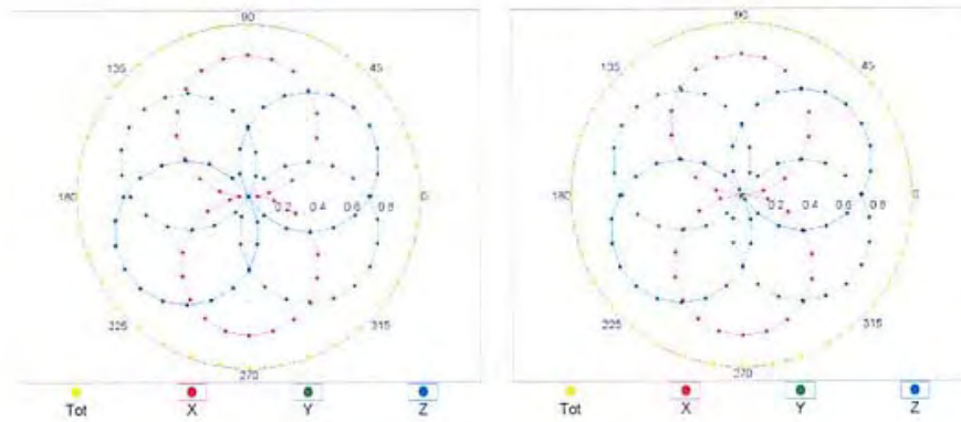
f=600 MHz,TEM
